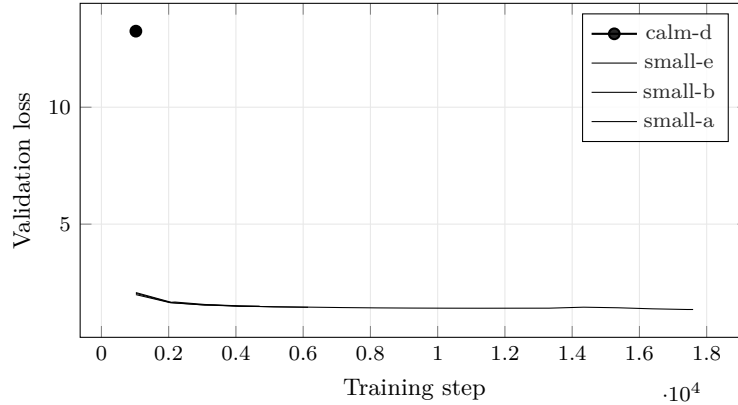
Figure 6: Validation Loss across the 4 most recent experiments with comparable validation curves; the leading run (calm-d) is drawn in bold. Generated from run logs - metrics that are not comparable across families (token loss vs. byte bits-per-byte vs. codec/CALM BrierLM) are excluded by construction, so the curves on this axis mean the same thing.
