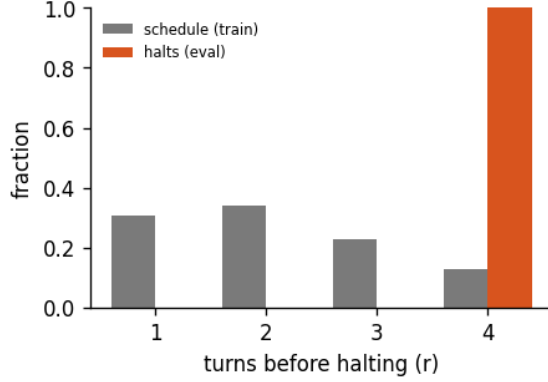
Figure 4: Halting distribution: the fraction of forward passes that stop after r turns, for the 4-turn recurrent loop of run calm-e, early-halt rate 0%, mean boundary KL 6.57. schedule is the random loop-count the model trains under; halts is where the KL gate actually stops at inference. A mass pinned at the maximum (KL never collapsing) is the honest signature of a model that has not yet learned to converge early - the decision is real, not yet decisive.
