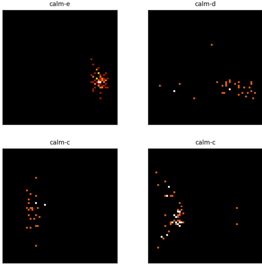
Figure 2: Center PCA density for the 4 most recent crystal-head runs (calm-e, calm-d, calm-c, calm-c). Each panel is the top-2 PCA projection of a head’s vocabulary centers, binned to a 64 \times 64 density grid (log color) - the same snapshot the dashboard renders live. Different runs settle into structurally different geometries, not noise.
