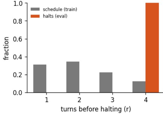
Figure 5: Halting distribution: the fraction of forward passes that stop after r turns, for the 4-turn recurrent loop of run calm-e, early-halt rate 0%, mean boundary KL 105. schedule is the random loop-count the model trains under; halts is where the KL gate actually stops at inference. A mass pinned at the maximum (KL never collapsing) is the honest signature of a model that has not yet learned to converge early - the decision is real, not yet decisive.
