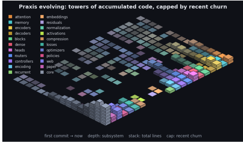
Figure 4: Praxis’s git history as an isometric terrain over the last 2280 commits. Each cell is one subsystem in one time window: a stack of base blocks for its accumulated size (total lines, recency-weighted) topped by a vivid cap for that window’s line churn - the standing codebase carrying the recent activity. Both are weighted by recency (the kernel the model applies to a sequence, turned on the repository): recent windows stack tall with bright caps while history thins toward the always-present prior - the low valley we roll into. Color fades from each subsystem’s hue toward a neutral prior into the past, banded in phased strata over a non-linear timescale. It is the bias/variance geometry read along the frequency axis (see the project notes): loud recent corrections over the quiet, ever-present base. By recency-weighted churn the current center of gravity is core, web, encoders. The framework charts the hand that builds it.
