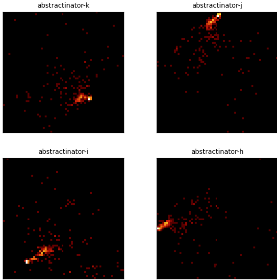
Figure 12: Center PCA density for the 4 most recent crystal-head runs ( abstractinator-k , abstractinator-j , abstractinator-i , abstractinator-h ). Each panel is the top-2 PCA projection of a head's vocabulary centers, binned to a 64 \times 64 density grid (log color) - the same snapshot the dashboard renders live. Different runs settle into structurally different geometries, not noise.
