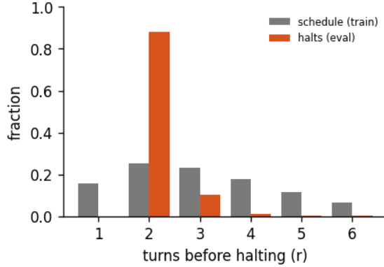
Figure 9: Halting distribution: the fraction of forward passes that stop after r turns, for the 6-turn recurrent loop of run abstractinator-u, early-halt rate 47%, mean boundary KL 0.675. schedule is the random loop-count the model trains under; halts is where the KL gate actually stops at inference. A mass pinned at the maximum (KL never collapsing) is the honest signature of a model that has not yet learned to converge early - the decision is real, not yet decisive.
