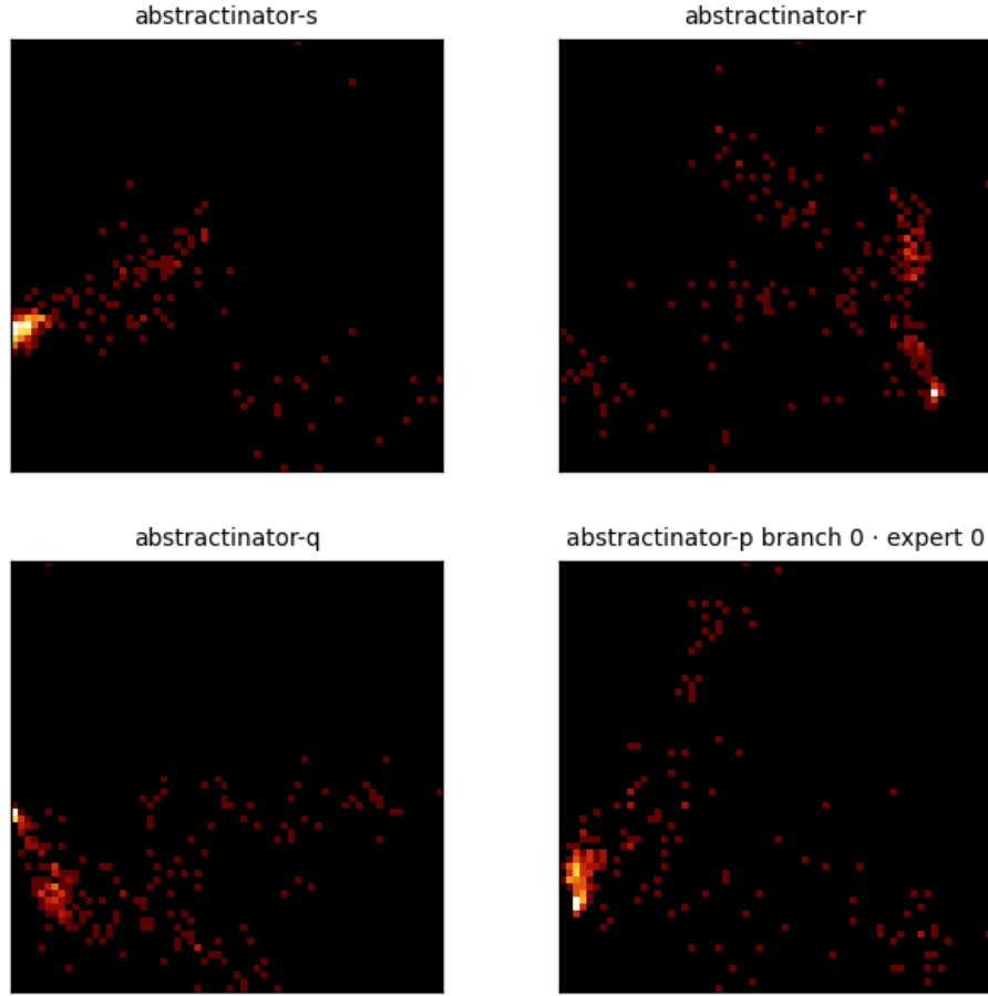
Figure 11: Center PCA density for the 4 most recent crystal-head runs ( abstractinator-s , abstractinator-r , abstractinator-q , abstractinator-p (branch 0 · expert 0)). Each panel is the top-2 PCA projection of a head’s vocabulary centers, binned to a 64 \times 64 density grid (log color) - the same snapshot the dashboard renders live. Different runs settle into structurally different geometries, not noise.
