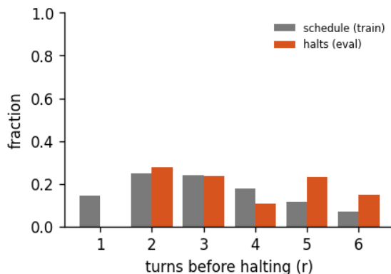
Figure 8: Halting distribution: the fraction of forward passes that stop after r turns, for the 6-turn recurrent loop of run abstractinator-s, early-halt rate 24%, mean boundary KL 0.336. schedule is the random loop-count the model trains under; halts is where the KL gate actually stops at inference. A mass pinned at the maximum (KL never collapsing) is the honest signature of a model that has not yet learned to converge early - the decision is real, not yet decisive.
