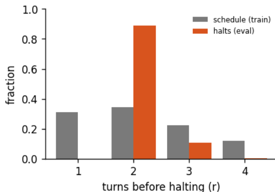
Figure 8: Halting distribution: the fraction of forward passes that stop after r turns, for the 4-turn recurrent loop of run abstractinator-f, early-halt rate 47%, mean boundary KL 0.424. schedule is the random loop-count the model trains under; halts is where the KL gate actually stops at inference. A mass pinned at the maximum (KL never collapsing) is the honest signature of a model that has not yet learned to converge early - the decision is real, not yet decisive.
