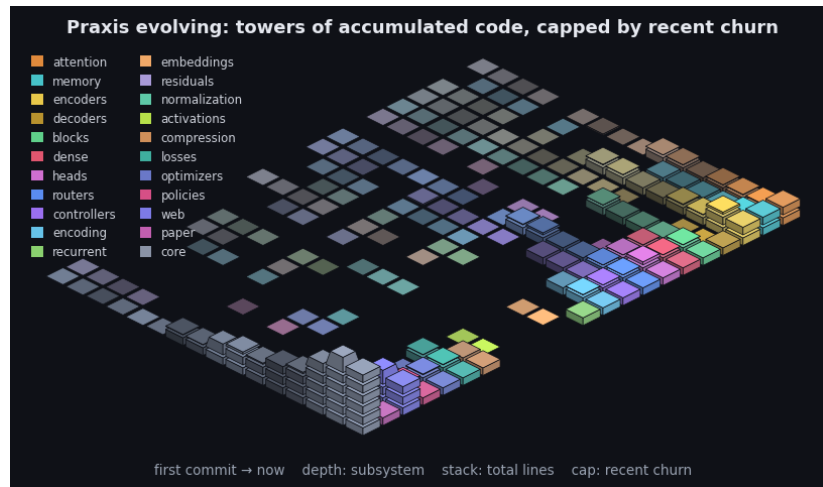
Figure 7: Praxis’s git history as an isometric terrain over the last 2219 commits. Each cell is one subsystem in one time window: a stack of base blocks for its accumulated size (total lines, recency-weighted) topped by a vivid cap for that window’s line churn - the standing codebase carrying the recent activity. Both are weighted by recency (the kernel the model applies to a sequence, turned on the repository): recent windows stack tall with bright caps while history thins toward the always-present prior - the low valley we roll into. Color fades from each subsystem’s hue toward a neutral prior into the past, banded in phased strata over a non-linear timescale. It is the bias/variance geometry read along the frequency axis (see the project notes): loud recent corrections over the quiet, ever-present base. By recency-weighted churn the current center of gravity is core, web, encoders. The framework charts the hand that builds it.
