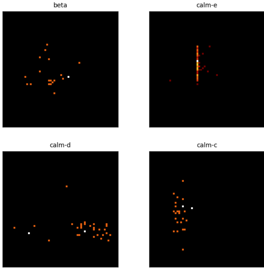
Figure 2: Center PCA density for the 4 most recent crystal-head runs (beta, calm-e, calm-d, calm-c). Each panel is the top-2 PCA projection of a head's vocabulary centers, binned to a 64 \times 64 density grid (log color) - the same snapshot the dashboard renders live. Different runs settle into structurally different geometries, not noise.
