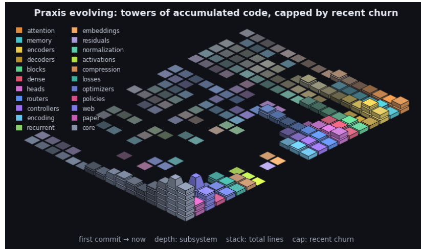
Figure 9: Praxis’s git history as an isometric terrain over the last 2363 commits. Each cell is one subsystem in one time window: a stack of base blocks for its accumulated size (total lines, recency-weighted) topped by a vivid cap for that window’s line churn - the standing codebase carrying the recent activity. Both are weighted by recency (the kernel the model applies to a sequence, turned on the repository): recent windows stack tall with bright caps while history thins toward the always-present prior - the low valley we roll into. Color fades from each subsystem’s hue toward a neutral prior into the past, banded in phased strata over a non-linear timescale. It is the bias/variance geometry read along the frequency axis (see the project notes): loud recent corrections over the quiet, ever-present base. By recency-weighted churn the current center of gravity is core, web, paper. The framework charts the hand that builds it.
