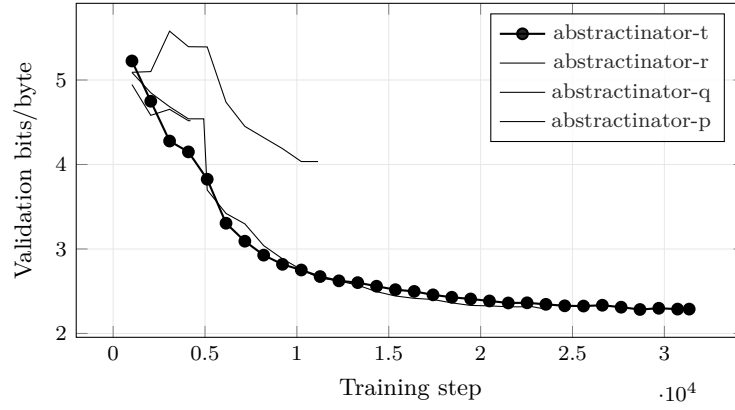
Figure 14: Bits per Byte across the 4 most recent experiments with comparable validation curves; the current experiment (abstractinator-t) is drawn in bold. Bold marks which run this build is reporting on , not which run scores best. The curves end wherever each run stopped, so they are at different points along their own training, and their endpoints are not a ranking. Generated from run logs - metrics that are not comparable across families (token loss vs. byte bits-per-byte vs. codec/CALM BrierLM) are excluded by construction, so the curves on this axis mean the same thing.
