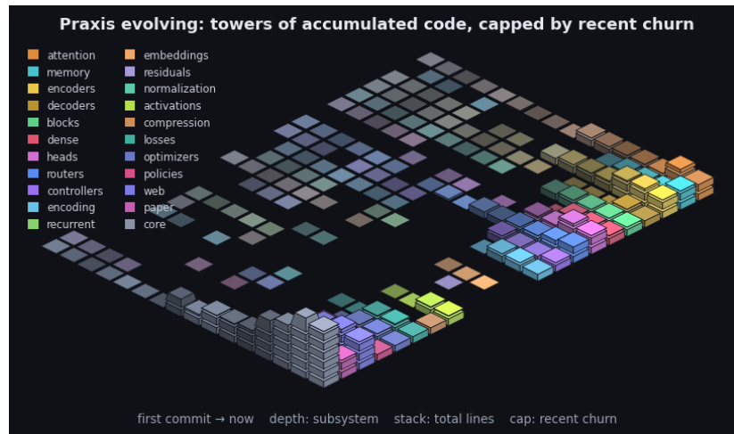
Figure 13: Praxis’s git history as an isometric terrain over the last 2594 commits. Each cell is one subsystem in one time window: a stack of base blocks for its accumulated size (total lines, recency-weighted) topped by a vivid cap for that window’s line churn - the standing codebase carrying the recent activity. Both are weighted by recency (the kernel the model applies to a sequence, turned on the repository): recent windows stack tall with bright caps while history thins toward the always-present prior - the low valley we roll into. Color fades from each subsystem’s hue toward a neutral prior into the past, banded in phased strata over a non-linear timescale. It is the bias/variance geometry read along the frequency axis (see the project notes): loud recent corrections over the quiet, ever-present base. By recency-weighted churn the current center of gravity is core, web, paper. The framework charts the hand that builds it.
