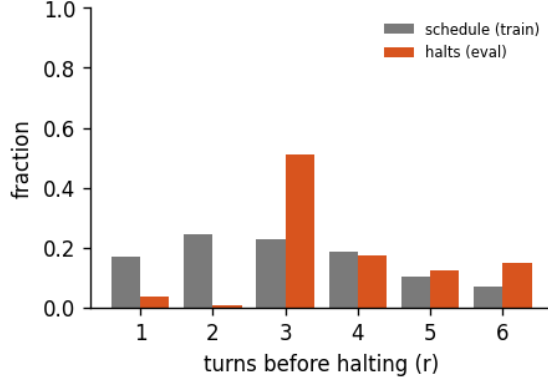
Figure 9: Halting distribution: the fraction of forward passes that stop after r turns, for the 6-turn recurrent loop of run abstractinator-u, early-halt rate 23%, mean boundary KL 0.178. schedule is the random loop-count the model trains under; halts is where the KL gate actually stops at inference. A mass pinned at the maximum (KL never collapsing) is the honest signature of a model that has not yet learned to converge early - the decision is real, not yet decisive.
