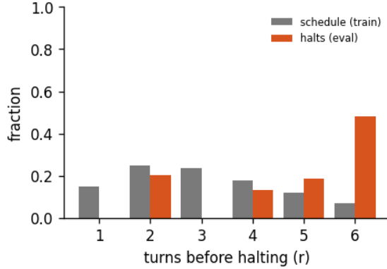
Figure 8: Halting distribution: the fraction of forward passes that stop after r turns, for the 6-turn recurrent loop of run abstractinator-m, early-halt rate 12%, mean boundary KL 0.382. schedule is the random loop-count the model trains under; halts is where the KL gate actually stops at inference. A mass pinned at the maximum (KL never collapsing) is the honest signature of a model that has not yet learned to converge early - the decision is real, not yet decisive.
