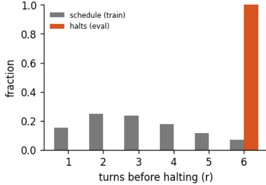
Figure 5: Halting distribution: the fraction of forward passes that stop after r turns, for the 6-turn recurrent loop of run calm-e, early-halt rate 0%, mean boundary KL 77.2. schedule is the random loop-count the model trains under; halts is where the KL gate actually stops at inference. A mass pinned at the maximum (KL never collapsing) is the honest signature of a model that has not yet learned to converge early - the decision is real, not yet decisive.
