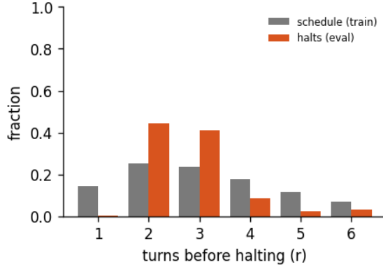
Figure 8: Halting distribution: the fraction of forward passes that stop after r turns, for the 6-turn recurrent loop of run abstractinator-n, early-halt rate 35%, mean boundary KL 0.178. schedule is the random loop-count the model trains under; halts is where the KL gate actually stops at inference. A mass pinned at the maximum (KL never collapsing) is the honest signature of a model that has not yet learned to converge early - the decision is real, not yet decisive.
