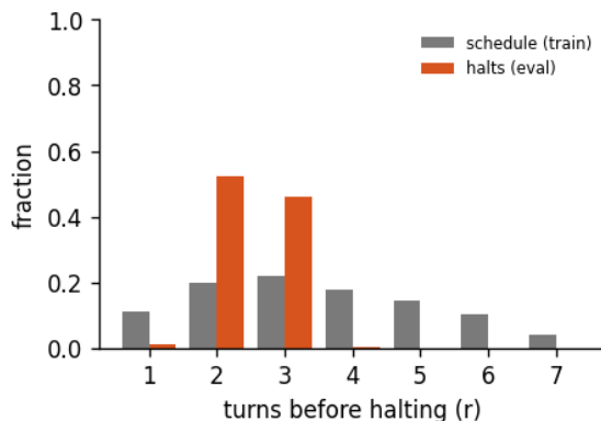
Figure 7: Halting distribution: the fraction of forward passes that stop after r turns, for the 7-turn recurrent loop of run abstractinator-c, early-halt rate 41%, mean boundary KL 0.272. schedule is the random loop-count the model trains under; halts is where the KL gate actually stops at inference. A mass pinned at the maximum (KL never collapsing) is the honest signature of a model that has not yet learned to converge early - the decision is real, not yet decisive.
