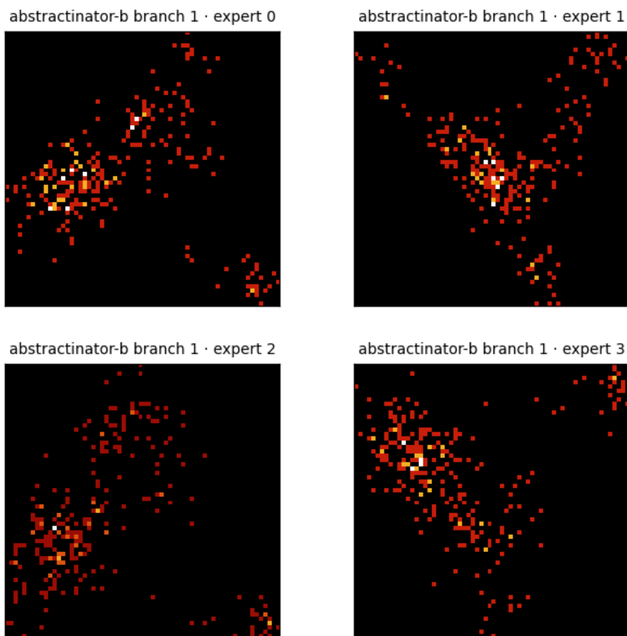
Figure 10: Center PCA density for the 4 crystal heads of abstractinator-b - a single multi-head model (prismatic4’s VEAR crystal bank), so these are that run’s own heads (branch 1 · expert 0, branch 1 · expert 1, branch 1 · expert 2, branch 1 · expert 3), not a cross-run mix. Each panel is the top-2 PCA projection of a head’s vocabulary centers, binned to a 64 \times 64 density grid (log color) - the same snapshot the dashboard renders live. The bank’s experts settle into structurally distinct geometries - the between-expert variance the router selects over.
