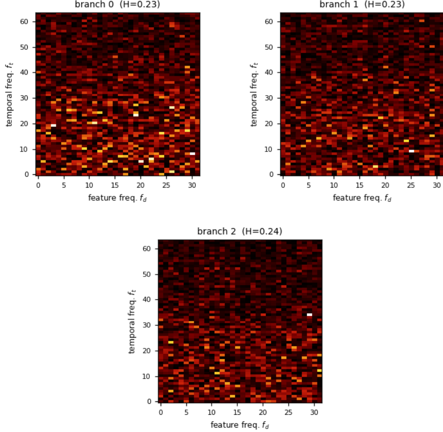
Figure 2: The static amplitude spectrum |a[f_t, f_d]| across the 3 arms of abstractinator-c’s prismatic head - the learned grid that, inverse-transformed through the frozen Weyl phases, becomes the bias field. This is the heatmap the text describes: energy that settles into a low-frequency band (small f_t, f_d ) is the corpus rhythm crystallizing, while a grid that stays uniform is a field still indistinguishable from noise. Hoyer concentrations H = 0.23, 0.23, 0.24 (left to right) quantifies it on the same [0, 1] scale the prose names (1 = a single cell, 0 = uniform), computed from this very tensor by concentration() - the same value the dashboard logs live. The pink 1/f^\alpha prior lives in the frozen basis, not in these amplitudes, so the grid shown is exactly what the head exposes.
