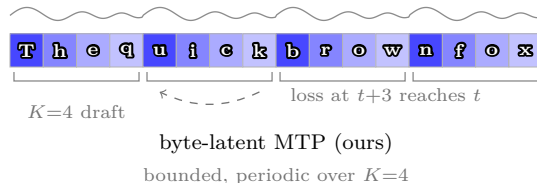
Figure 4: The fox in windows: the strip of Figure 6, reorganized as this run’s generation reads it - draft windows of K=4 bytes, each carrying its own short curve. Shade is the within-window density profile the acceptance metric measures: heavy where the draft is fresh off the trunk state, thinning as draft depth grows, restarting at every reseed. The dashed return is the training-time coupling that makes the window a curve rather than four independent points: all four losses land on one state, so supervision at the window’s tip reaches its head. Where the continuous-latent program raises one unbounded field over the whole sequence, this head repeats a small periodic one - the same dependence, contained. Schematic, not measured; the measured object is the per-depth acceptance profile.
