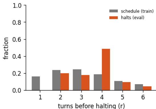
Figure 8: Halting distribution: the fraction of forward passes that stop after r turns, for the 6-turn recurrent loop of run abstractinator-g, early-halt rate 27%, mean boundary KL 0.248. schedule is the random loop-count the model trains under; halts is where the KL gate actually stops at inference. A mass pinned at the maximum (KL never collapsing) is the honest signature of a model that has not yet learned to converge early - the decision is real, not yet decisive.
