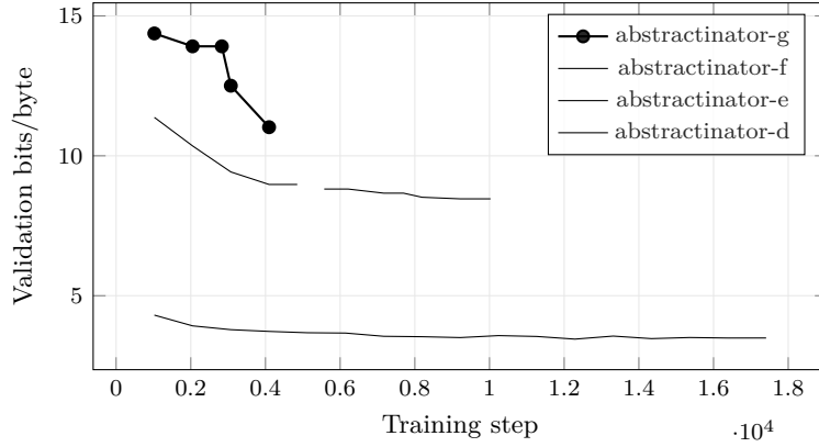
Figure 13: Bits per Byte across the 4 most recent experiments with comparable validation curves; the current experiment (abstractinator-g) is drawn in bold. Bold marks which run this build is reporting on , not which run scores best. The curves end wherever each run stopped, so they are at different points along their own training, and their endpoints are not a ranking. Generated from run logs - metrics that are not comparable across families (token loss vs. byte bits-per-byte vs. codec/CALM BrierLM) are excluded by construction, so the curves on this axis mean the same thing.
