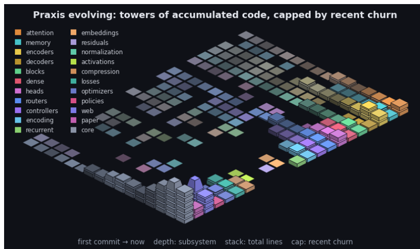
Figure 4: Praxis’s git history as an isometric terrain over the last 2333 commits. Each cell is one subsystem in one time window: a stack of base blocks for its accumulated size (total lines, recency-weighted) topped by a vivid cap for that window’s line churn - the standing codebase carrying the recent activity. Both are weighted by recency (the kernel the model applies to a sequence, turned on the repository): recent windows stack tall with bright caps while history thins toward the always-present prior - the low valley we roll into. Color fades from each subsystem’s hue toward a neutral prior into the past, banded in phased strata over a non-linear timescale. It is the bias/variance geometry read along the frequency axis (see the project notes): loud recent corrections over the quiet, ever-present base. By recency-weighted churn the current center of gravity is core, web, paper. The framework charts the hand that builds it.
