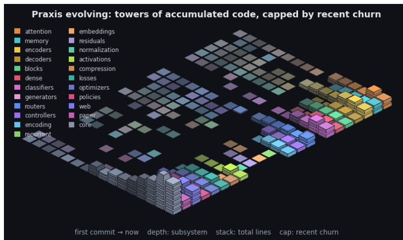
Figure 9: Praxis’s git history as an isometric terrain over the last 2681 commits. Each cell is one subsystem in one time window: a stack of base blocks for its accumulated size (total lines, recency-weighted) topped by a vivid cap for that window’s line churn - the standing codebase carrying the recent activity. Both are weighted by recency (the kernel the model applies to a sequence, turned on the repository): recent windows stack tall with bright caps while history thins toward the always-present prior - the low valley we roll into. Color fades from each subsystem’s hue toward a neutral prior into the past, banded in phased strata over a non-linear timescale. It is the bias/variance geometry read along the frequency axis (see the project notes): loud recent corrections over the quiet, ever-present base. By recency-weighted churn the current center of gravity is core, web, encoders. The framework charts the hand that builds it.
