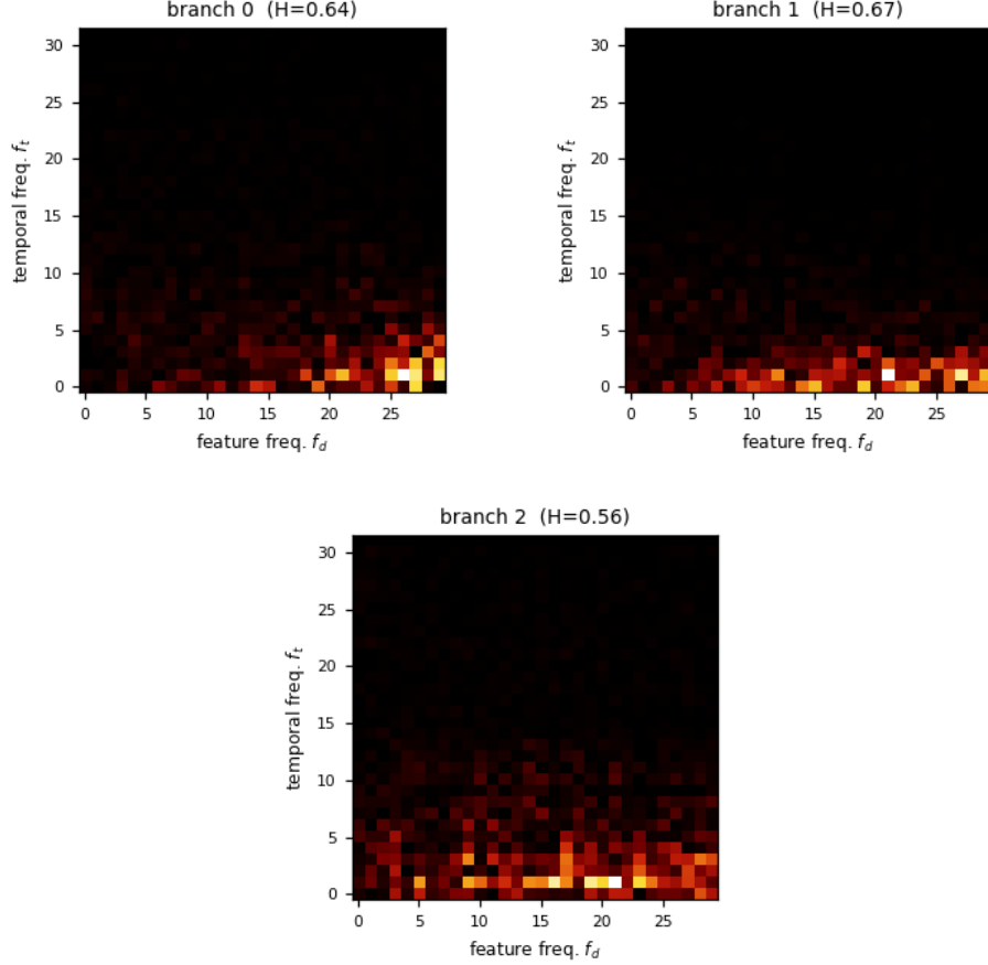
Figure 2: The static amplitude spectrum |a[f_t, f_d]| across the 3 arms of abstractinator-e’s prismatic head - the learned grid that, inverse-transformed through the frozen Weyl phases, becomes the bias field. This is the heatmap the text describes: energy that settles into a low-frequency band (small f_t, f_d ) is the corpus rhythm crystallizing, while a grid that stays uniform is a field still indistinguishable from noise. Hoyer concentrations H = 0.64, 0.67, 0.56 (left to right) quantifies it on the same [0, 1] scale the prose names (1 = a single cell, 0 = uniform), computed from this very tensor by concentration() - the same value the dashboard logs live. The pink 1/f^\alpha prior lives in the frozen basis, not in these amplitudes, so the grid shown is exactly what the head exposes.
