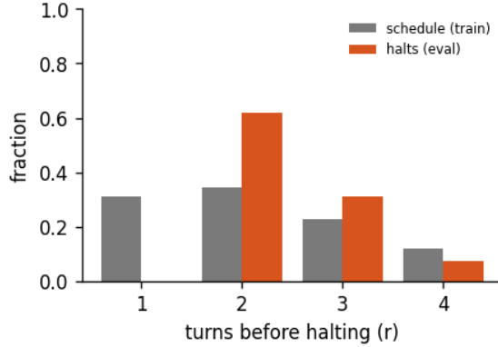
Figure 7: Halting distribution: the fraction of forward passes that stop after r turns, for the 4-turn recurrent loop of run abstractinator-e, early-halt rate 39%, mean boundary KL 0.451. schedule is the random loop-count the model trains under; halts is where the KL gate actually stops at inference. A mass pinned at the maximum (KL never collapsing) is the honest signature of a model that has not yet learned to converge early - the decision is real, not yet decisive.
