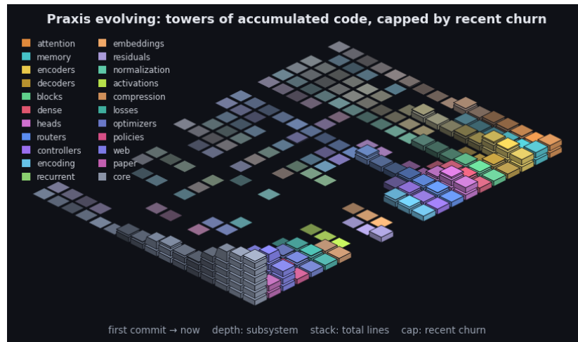
Figure 11: Praxis’s git history as an isometric terrain over the last 2435 commits. Each cell is one subsystem in one time window: a stack of base blocks for its accumulated size (total lines, recency-weighted) topped by a vivid cap for that window’s line churn - the standing codebase carrying the recent activity. Both are weighted by recency (the kernel the model applies to a sequence, turned on the repository): recent windows stack tall with bright caps while history thins toward the always-present prior - the low valley we roll into. Color fades from each subsystem’s hue toward a neutral prior into the past, banded in phased strata over a non-linear timescale. It is the bias/variance geometry read along the frequency axis (see the project notes): loud recent corrections over the quiet, ever-present base. By recency-weighted churn the current center of gravity is core, web, paper. The framework charts the hand that builds it.
