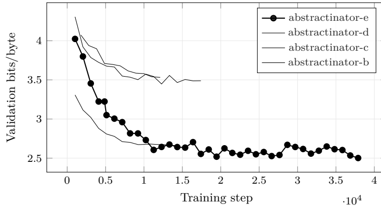
Figure 12: Bits per Byte across the 4 most recent experiments with comparable validation curves; the leading run (abstractinator-e) is drawn in bold. Generated from run logs - metrics that are not comparable across families (token loss vs. byte bits-per-byte vs. codec/CALM BrierLM) are excluded by construction, so the curves on this axis mean the same thing.
