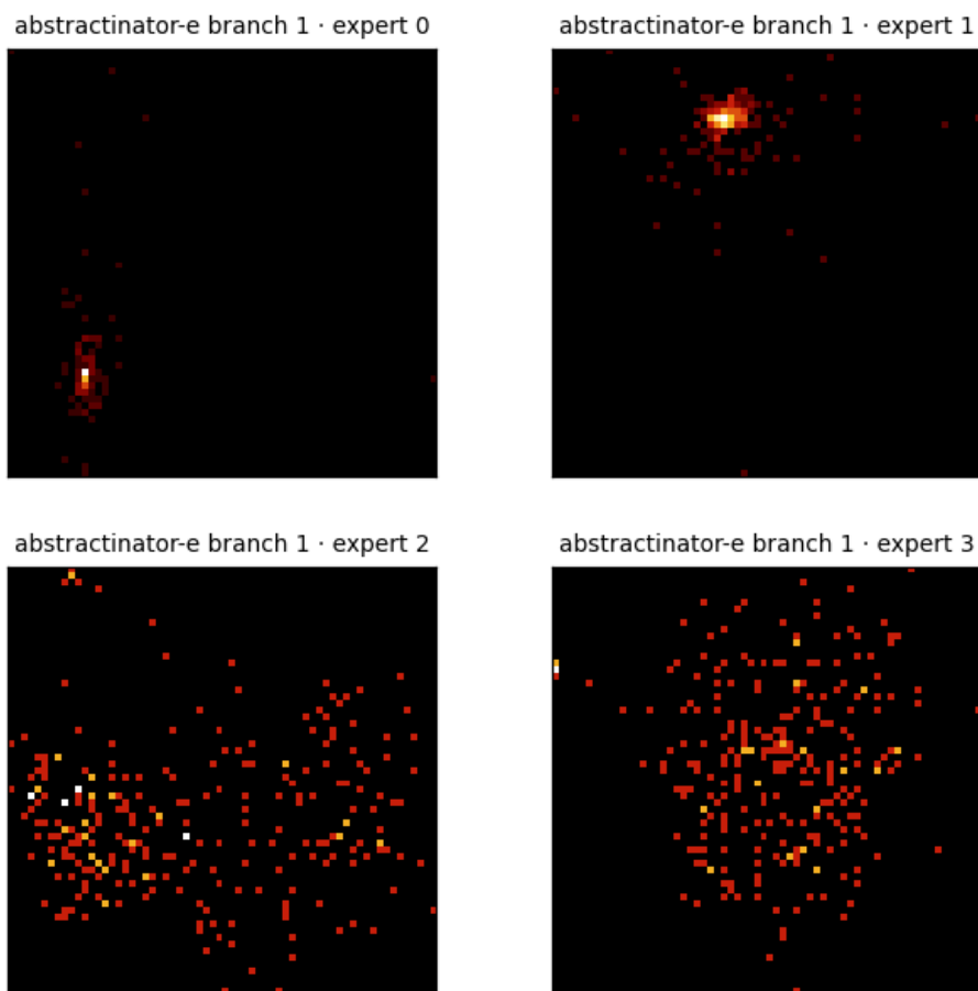
Figure 10: Center PCA density for the 4 crystal heads of abstractinator-e - a single multi-head model (prismatic4’s VEAR crystal bank), so these are that run’s own heads (branch 1 · expert 0, branch 1 · expert 1, branch 1 · expert 2, branch 1 · expert 3), not a cross-run mix. Each panel is the top-2 PCA projection of a head’s vocabulary centers, binned to a 64 \times 64 density grid (log color) - the same snapshot the dashboard renders live. The bank’s experts settle into structurally distinct geometries - the between-expert variance the router selects over.
