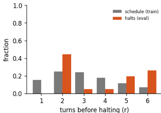
Figure 8: Halting distribution: the fraction of forward passes that stop after r turns, for the 6-turn recurrent loop of run abstractinator-r, early-halt rate 21%, mean boundary KL 0.545. schedule is the random loop-count the model trains under; halts is where the KL gate actually stops at inference. A mass pinned at the maximum (KL never collapsing) is the honest signature of a model that has not yet learned to converge early - the decision is real, not yet decisive.
