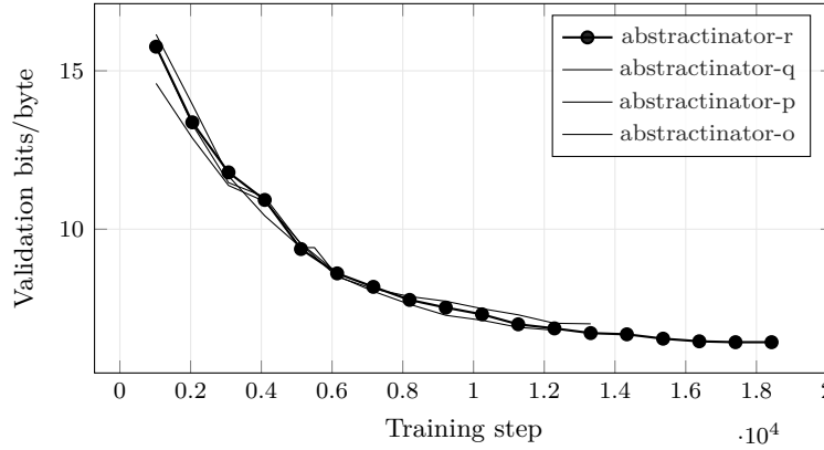
Figure 13: Bits per Byte across the 4 most recent experiments with comparable validation curves; the current experiment (abstractinator-r) is drawn in bold. Bold marks which run this build is reporting on , not which run scores best. The curves end wherever each run stopped, so they are at different points along their own training, and their endpoints are not a ranking. Generated from run logs - metrics that are not comparable across families (token loss vs. byte bits-per-byte vs. codec/CALM BrierLM) are excluded by construction, so the curves on this axis mean the same thing.
