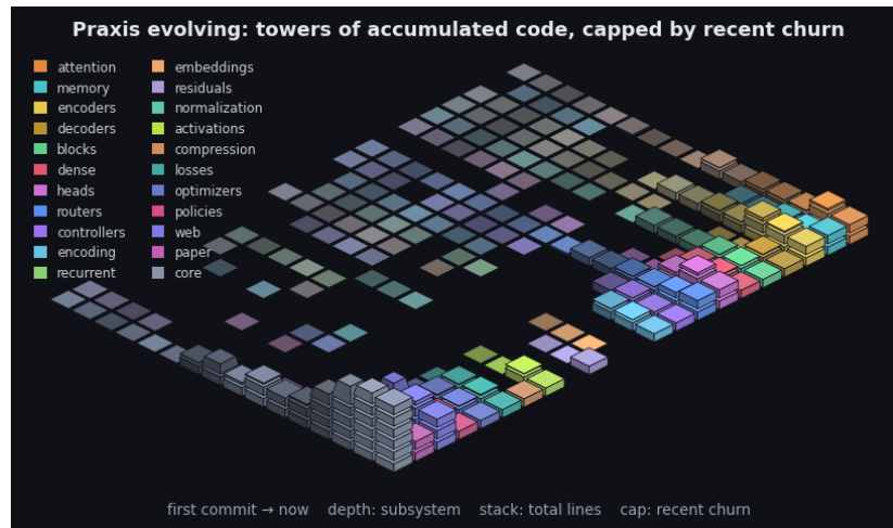
Figure 12: Praxis’s git history as an isometric terrain over the last 2529 commits. Each cell is one subsystem in one time window: a stack of base blocks for its accumulated size (total lines, recency-weighted) topped by a vivid cap for that window’s line churn - the standing codebase carrying the recent activity. Both are weighted by recency (the kernel the model applies to a sequence, turned on the repository): recent windows stack tall with bright caps while history thins toward the always-present prior - the low valley we roll into. Color fades from each subsystem’s hue toward a neutral prior into the past, banded in phased strata over a non-linear timescale. It is the bias/variance geometry read along the frequency axis (see the project notes): loud recent corrections over the quiet, ever-present base. By recency-weighted churn the current center of gravity is core, web, paper. The framework charts the hand that builds it.
