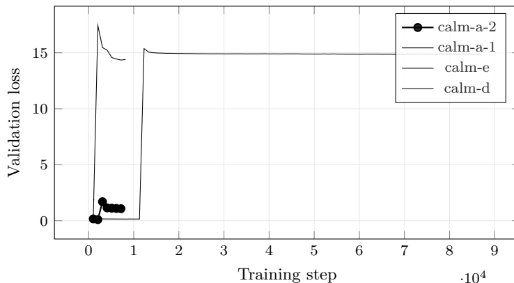
Figure 5: Validation Loss across the 4 most recent experiments with comparable validation curves; the leading run ( calm-a-2 ) is drawn in bold. Generated from run logs - metrics that are not comparable across families (token loss vs. byte bits-per-byte vs. codec/CALM BrierLM) are excluded by construction, so the curves on this axis mean the same thing.
