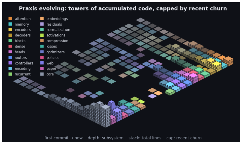
Figure 4: Praxis’s git history as an isometric terrain over the last 2324 commits. Each cell is one subsystem in one time window: a stack of base blocks for its accumulated size (total lines, recency-weighted) topped by a vivid cap for that window’s line churn - the standing codebase carrying the recent activity. Both are weighted by recency (the kernel the model applies to a sequence, turned on the repository): recent windows stack tall with bright caps while history thins toward the always-present prior - the low valley we roll into. Color fades from each subsystem’s hue toward a neutral prior into the past, banded in phased strata over a non-linear timescale. It is the bias/variance geometry read along the frequency axis (see the project notes): loud recent corrections over the quiet, ever-present base. By recency-weighted churn the current center of gravity is core, web, paper. The framework charts the hand that builds it.
