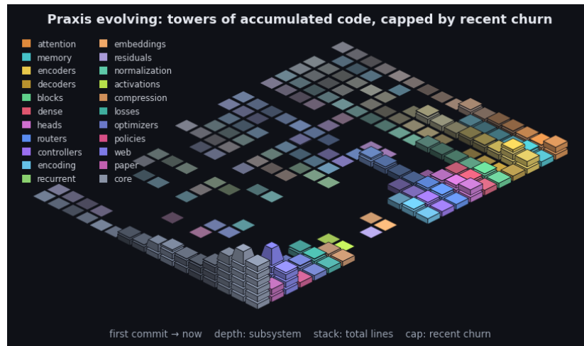
Figure 10: Praxis's git history as an isometric terrain over the last 2383 commits. Each cell is one subsystem in one time window: a stack of base blocks for its accumulated size (total lines, recency-weighted) topped by a vivid cap for that window's line churn - the standing codebase carrying the recent activity. Both are weighted by recency (the kernel the model applies to a sequence, turned on the repository): recent windows stack tall with bright caps while history thins toward the always-present prior - the low valley we roll into. Color fades from each subsystem's hue toward a neutral prior into the past, banded in phased strata over a non-linear timescale. It is the bias/variance geometry read along the frequency axis (see the project notes): loud recent corrections over the quiet, ever-present base. By recency-weighted churn the current center of gravity is core, web, paper. The framework charts the hand that builds it.
