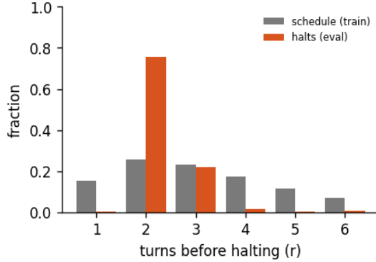
Figure 8: Halting distribution: the fraction of forward passes that stop after r turns, for the 6-turn recurrent loop of run abstractinator-i, early-halt rate 44%, mean boundary KL 1.17. schedule is the random loop-count the model trains under; halts is where the KL gate actually stops at inference. A mass pinned at the maximum (KL never collapsing) is the honest signature of a model that has not yet learned to converge early - the decision is real, not yet decisive.
