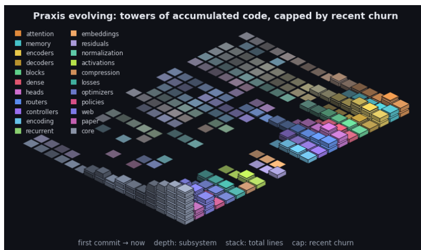
Figure 12: Praxis’s git history as an isometric terrain over the last 2555 commits. Each cell is one subsystem in one time window: a stack of base blocks for its accumulated size (total lines, recency-weighted) topped by a vivid cap for that window’s line churn - the standing codebase carrying the recent activity. Both are weighted by recency (the kernel the model applies to a sequence, turned on the repository): recent windows stack tall with bright caps while history thins toward the always-present prior - the low valley we roll into. Color fades from each subsystem’s hue toward a neutral prior into the past, banded in phased strata over a non-linear timescale. It is the bias/variance geometry read along the frequency axis (see the project notes): loud recent corrections over the quiet, ever-present base. By recency-weighted churn the current center of gravity is core, web, paper. The framework charts the hand that builds it.
