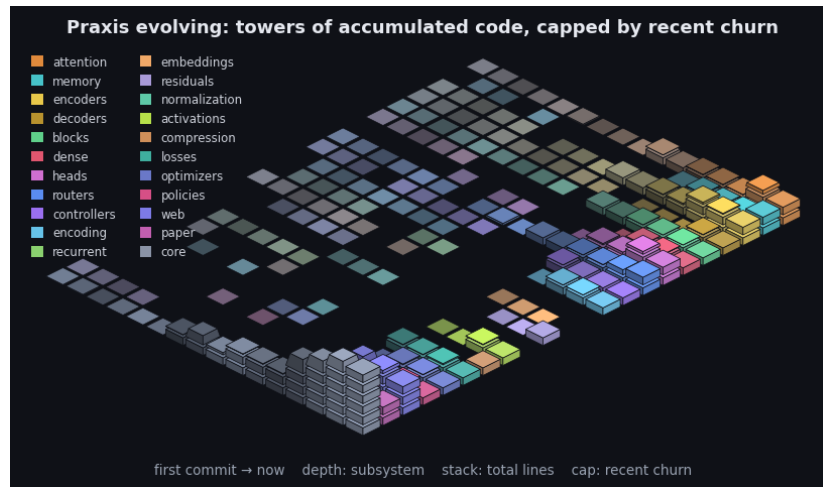
Figure 13: Praxis’s git history as an isometric terrain over the last 2563 commits. Each cell is one subsystem in one time window: a stack of base blocks for its accumulated size (total lines, recency-weighted) topped by a vivid cap for that window’s line churn - the standing codebase carrying the recent activity. Both are weighted by recency (the kernel the model applies to a sequence, turned on the repository): recent windows stack tall with bright caps while history thins toward the always-present prior - the low valley we roll into. Color fades from each subsystem’s hue toward a neutral prior into the past, banded in phased strata over a non-linear timescale. It is the bias/variance geometry read along the frequency axis (see the project notes): loud recent corrections over the quiet, ever-present base. By recency-weighted churn the current center of gravity is core, web, paper. The framework charts the hand that builds it.
