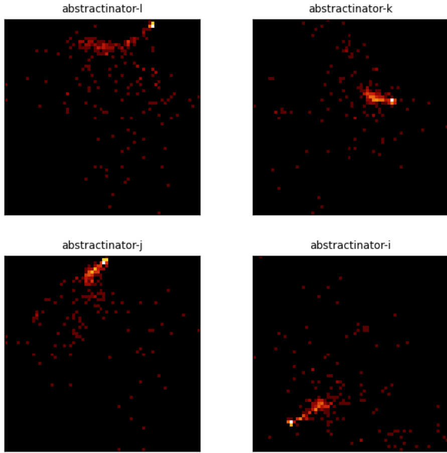
Figure 12: Center PCA density for the 4 most recent crystal-head runs ( abstractinator-l , abstractinator-k , abstractinator-j , abstractinator-i ). Each panel is the top-2 PCA projection of a head’s vocabulary centers, binned to a 64 \times 64 density grid (log color) - the same snapshot the dashboard renders live. Different runs settle into structurally different geometries, not noise.
