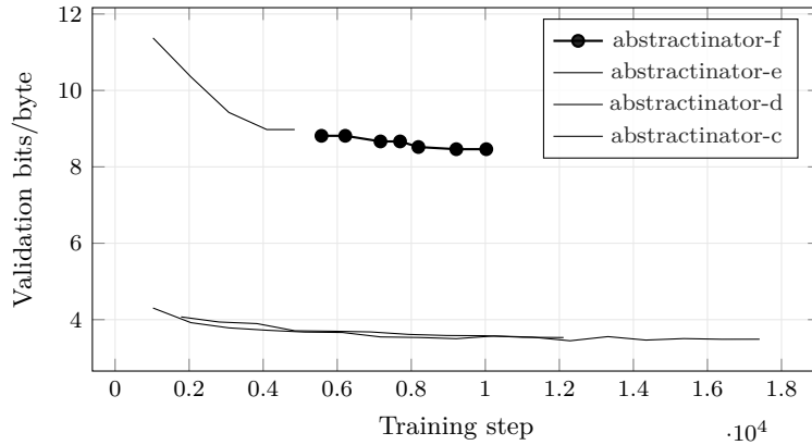
Figure 13: Bits per Byte across the 4 most recent experiments with comparable validation curves; the leading run (abstractinator-f) is drawn in bold. Generated from run logs - metrics that are not comparable across families (token loss vs. byte bits-per-byte vs. codec/CALM BrierLM) are excluded by construction, so the curves on this axis mean the same thing.
