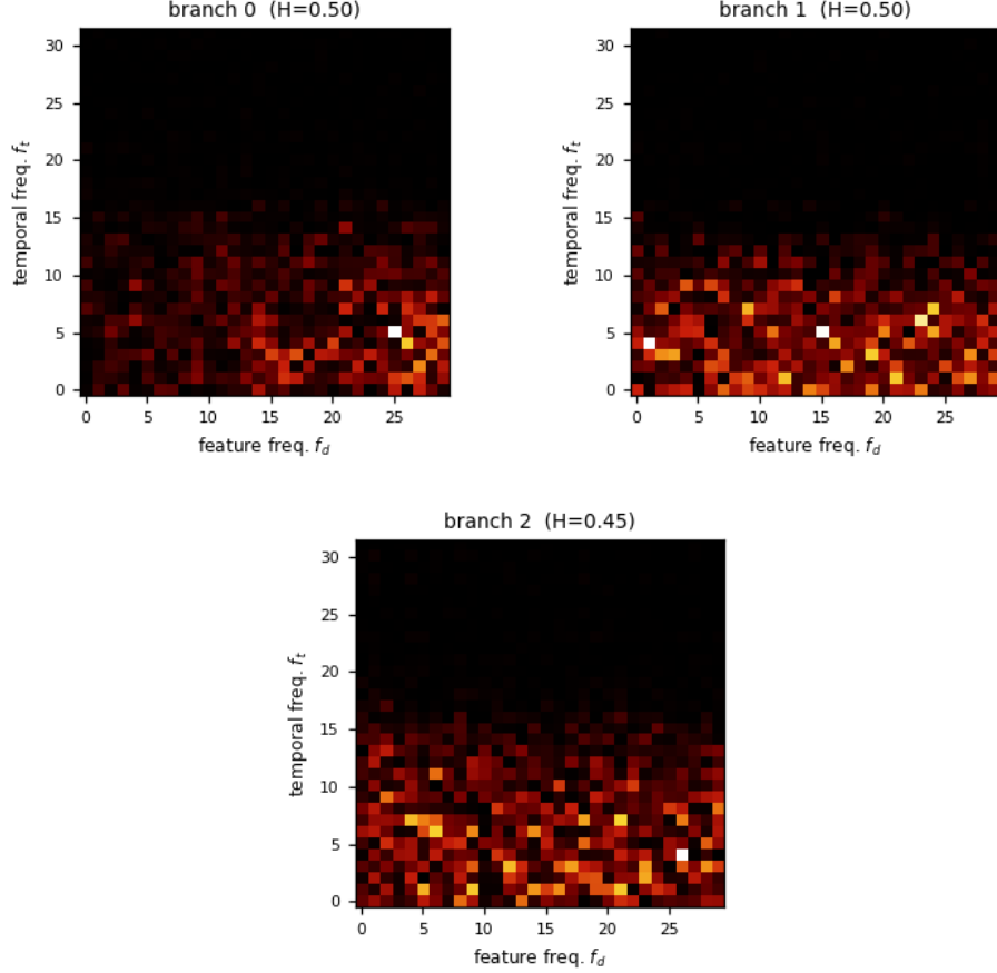
Figure 2: The static amplitude spectrum |a[f_t, f_d]| across the 3 arms of abstractinator-f's prismatic head - the learned grid that, inverse-transformed through the frozen Weyl phases, becomes the bias field. This is the heatmap the text describes: energy that settles into a low-frequency band (small f_t, f_d ) is the corpus rhythm crystallizing, while a grid that stays uniform is a field still indistinguishable from noise. Hoyer concentrations H = 0.50, 0.50, 0.45 (left to right) quantifies it on the same [0, 1] scale the prose names (1 = a single cell, 0 = uniform), computed from this very tensor by concentration() - the same value the dashboard logs live. The pink 1/f^\alpha prior lives in the frozen basis, not in these amplitudes, so the grid shown is exactly what the head exposes.
