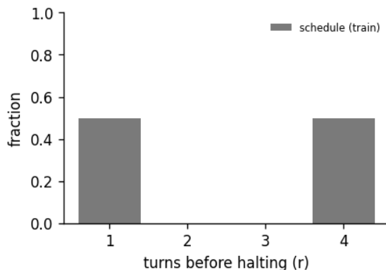
Figure 8: Halting distribution: the fraction of forward passes that stop after r turns, for the 4-turn recurrent loop of run abstractinator-g. schedule is the random loop-count the model trains under; halts is where the KL gate actually stops at inference. A mass pinned at the maximum (KL never collapsing) is the honest signature of a model that has not yet learned to converge early - the decision is real, not yet decisive.
