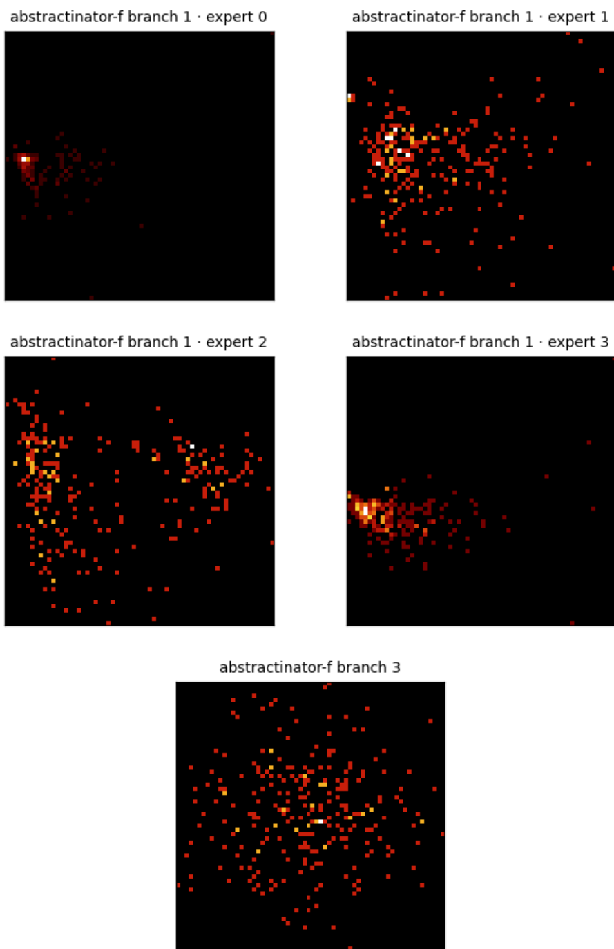
Figure 11: Center PCA density for the 5 crystal heads of abstractinator-f - a single multi-head model (prismatic4's VEAR crystal bank), so these are that run's own heads (branch 1 · expert 0, branch 1 · expert 1, branch 1 · expert 2, branch 1 · expert 3, branch 3), not a cross-run mix. Each panel is the top-2 PCA projection of a head's vocabulary centers, binned to a 64x64 density grid (log color) - the same snapshot the dashboard renders live. The bank's experts settle into structurally distinct geometries - the between-expert variance the router selects over.
