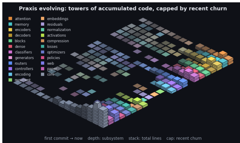
Figure 13: Praxis’s git history as an isometric terrain over the last 2649 commits. Each cell is one subsystem in one time window: a stack of base blocks for its accumulated size (total lines, recency-weighted) topped by a vivid cap for that window’s line churn - the standing codebase carrying the recent activity. Both are weighted by recency (the kernel the model applies to a sequence, turned on the repository): recent windows stack tall with bright caps while history thins toward the always-present prior - the low valley we roll into. Color fades from each subsystem’s hue toward a neutral prior into the past, banded in phased strata over a non-linear timescale. It is the bias/variance geometry read along the frequency axis (see the project notes): loud recent corrections over the quiet, ever-present base. By recency-weighted churn the current center of gravity is core, web, encoders. The framework charts the hand that builds it.
