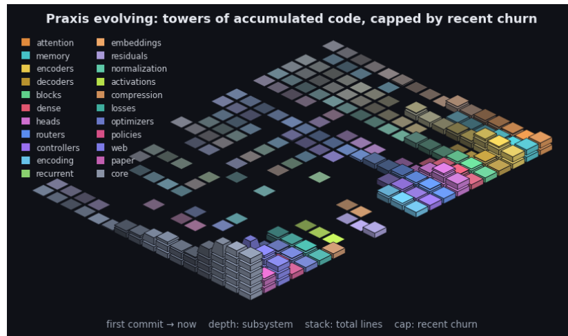
Figure 12: Praxis’s git history as an isometric terrain over the last 2460 commits. Each cell is one subsystem in one time window: a stack of base blocks for its accumulated size (total lines, recency-weighted) topped by a vivid cap for that window’s line churn - the standing codebase carrying the recent activity. Both are weighted by recency (the kernel the model applies to a sequence, turned on the repository): recent windows stack tall with bright caps while history thins toward the always-present prior - the low valley we roll into. Color fades from each subsystem’s hue toward a neutral prior into the past, banded in phased strata over a non-linear timescale. It is the bias/variance geometry read along the frequency axis (see the project notes): loud recent corrections over the quiet, ever-present base. By recency-weighted churn the current center of gravity is core, web, paper. The framework charts the hand that builds it.
