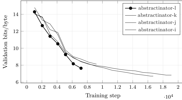
Figure 14: Bits per Byte across the 4 most recent experiments with comparable validation curves; the current experiment (abstractinator-l) is drawn in bold. Bold marks which run this build is reporting on , not which run scores best. The curves end wherever each run stopped, so they are at different points along their own training, and their endpoints are not a ranking. Generated from run logs - metrics that are not comparable across families (token loss vs. byte bits-per-byte vs. codec/CALM BrierLM) are excluded by construction, so the curves on this axis mean the same thing.
