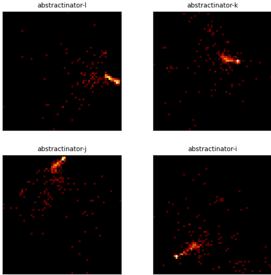
Figure 12: Center PCA density for the 4 most recent crystal-head runs (abstractinator-l, abstractinator-k, abstractinator-j, abstractinator-i). Each panel is the top-2 PCA projection of a head’s vocabulary centers, binned to a 64 \times 64 density grid (log color) - the same snapshot the dashboard renders live. Different runs settle into structurally different geometries, not noise.
