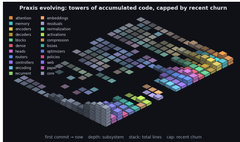
Figure 13: Praxis’s git history as an isometric terrain over the last 2562 commits. Each cell is one subsystem in one time window: a stack of base blocks for its accumulated size (total lines, recency-weighted) topped by a vivid cap for that window’s line churn - the standing codebase carrying the recent activity. Both are weighted by recency (the kernel the model applies to a sequence, turned on the repository): recent windows stack tall with bright caps while history thins toward the always-present prior - the low valley we roll into. Color fades from each subsystem’s hue toward a neutral prior into the past, banded in phased strata over a non-linear timescale. It is the bias/variance geometry read along the frequency axis (see the project notes): loud recent corrections over the quiet, ever-present base. By recency-weighted churn the current center of gravity is core, web, paper. The framework charts the hand that builds it.
