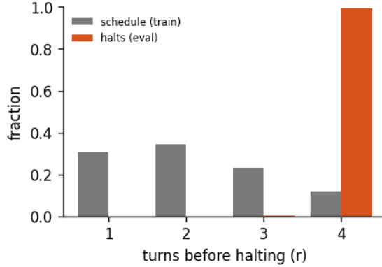
Figure 2: Halting distribution: the fraction of forward passes that stop after r turns, for the 4-turn recurrent loop of run calm-d-1, early-halt rate 0%, mean boundary KL 0.0713. schedule is the random loop-count the model trains under; halts is where the KL gate actually stops at inference. A mass pinned at the maximum (KL never collapsing) is the honest signature of a model that has not yet learned to converge early - the decision is real, not yet decisive.
