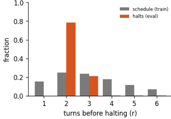
Figure 9: Halting distribution: the fraction of forward passes that stop after r turns, for the 6-turn recurrent loop of run abstractinator-n, early-halt rate 45%, mean boundary KL 0.924. schedule is the random loop-count the model trains under; halts is where the KL gate actually stops at inference. A mass pinned at the maximum (KL never collapsing) is the honest signature of a model that has not yet learned to converge early - the decision is real, not yet decisive.
