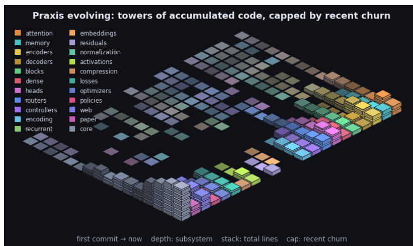
Figure 13: Praxis’s git history as an isometric terrain over the last 2567 commits. Each cell is one subsystem in one time window: a stack of base blocks for its accumulated size (total lines, recency-weighted) topped by a vivid cap for that window’s line churn - the standing codebase carrying the recent activity. Both are weighted by recency (the kernel the model applies to a sequence, turned on the repository): recent windows stack tall with bright caps while history thins toward the always-present prior - the low valley we roll into. Color fades from each subsystem’s hue toward a neutral prior into the past, banded in phased strata over a non-linear timescale. It is the bias/variance geometry read along the frequency axis (see the project notes): loud recent corrections over the quiet, ever-present base. By recency-weighted churn the current center of gravity is core, web, paper. The framework charts the hand that builds it.
