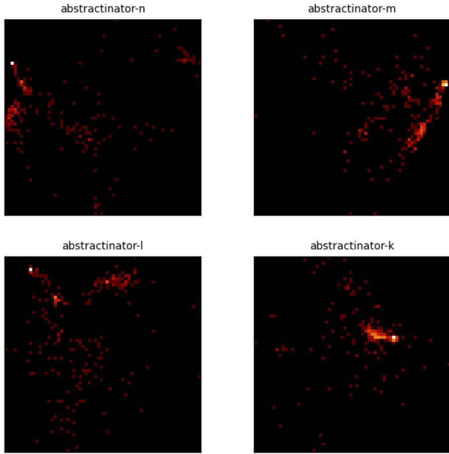
Figure 12: Center PCA density for the 4 most recent crystal-head runs ( abstractinator-n , abstractinator-m , abstractinator-l , abstractinator-k ). Each panel is the top-2 PCA projection of a head's vocabulary centers, binned to a 64 \times 64 density grid (log color) - the same snapshot the dashboard renders live. Different runs settle into structurally different geometries, not noise.
