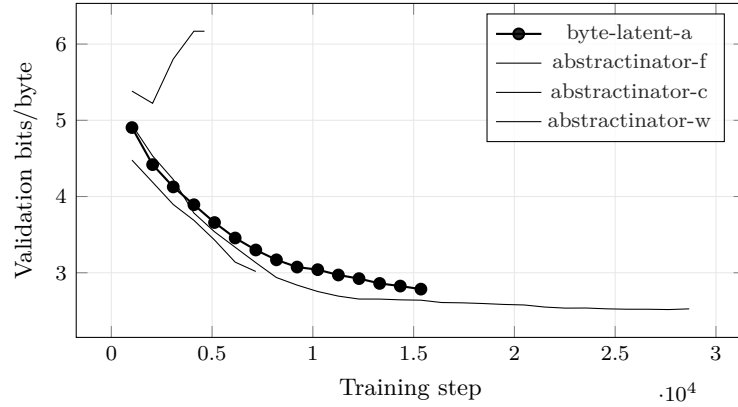
Figure 14: Bits per Byte across the 4 most recent experiments with comparable validation curves; the current experiment (byte-latent-a) is drawn in bold. Bold marks which run this build is reporting on , not which run scores best. The curves end wherever each run stopped, so they are at different points along their own training, and their endpoints are not a ranking. Generated from run logs - metrics that are not comparable across families (token loss vs. byte bits-per-byte vs. codec/CALM BrierLM) are excluded by construction, so the curves on this axis mean the same thing.
