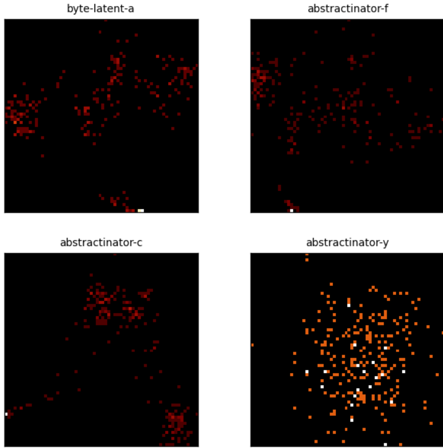
Figure 5: Center PCA density for the 4 most recent crystal-head runs (byte-latent-a, abstractinator-f, abstractinator-c, abstractinator-y). Each panel is the top-2 PCA projection of a head’s vocabulary centers, binned to a 64 \times 64 density grid (log color) - the same snapshot the dashboard renders live. Different runs settle into structurally different geometries, not noise.
