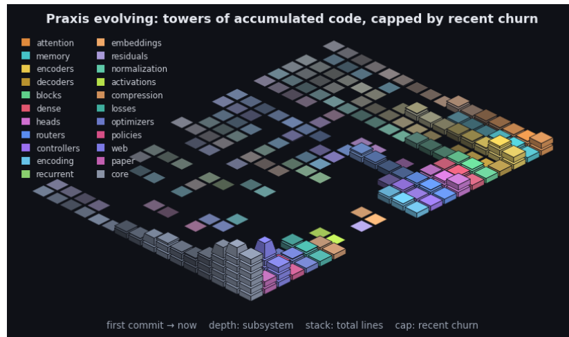
Figure 10: Praxis's git history as an isometric terrain over the last 2400 commits. Each cell is one subsystem in one time window: a stack of base blocks for its accumulated size (total lines, recency-weighted) topped by a vivid cap for that window's line churn - the standing codebase carrying the recent activity. Both are weighted by recency (the kernel the model applies to a sequence, turned on the repository): recent windows stack tall with bright caps while history thins toward the always-present prior - the low valley we roll into. Color fades from each subsystem's hue toward a neutral prior into the past, banded in phased strata over a non-linear timescale. It is the bias/variance geometry read along the frequency axis (see the project notes): loud recent corrections over the quiet, ever-present base. By recency-weighted churn the current center of gravity is core, web, paper. The framework charts the hand that builds it.
