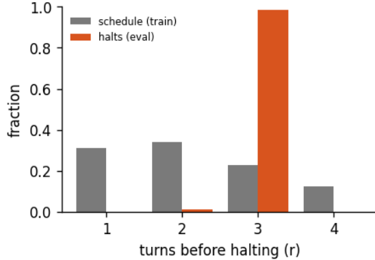
Figure 6: Halting distribution: the fraction of forward passes that stop after r turns, for the 4-turn recurrent loop of run calm-d-1, early-halt rate 33%, mean boundary KL 0.279. schedule is the random loop-count the model trains under; halts is where the KL gate actually stops at inference. A mass pinned at the maximum (KL never collapsing) is the honest signature of a model that has not yet learned to converge early - the decision is real, not yet decisive.
