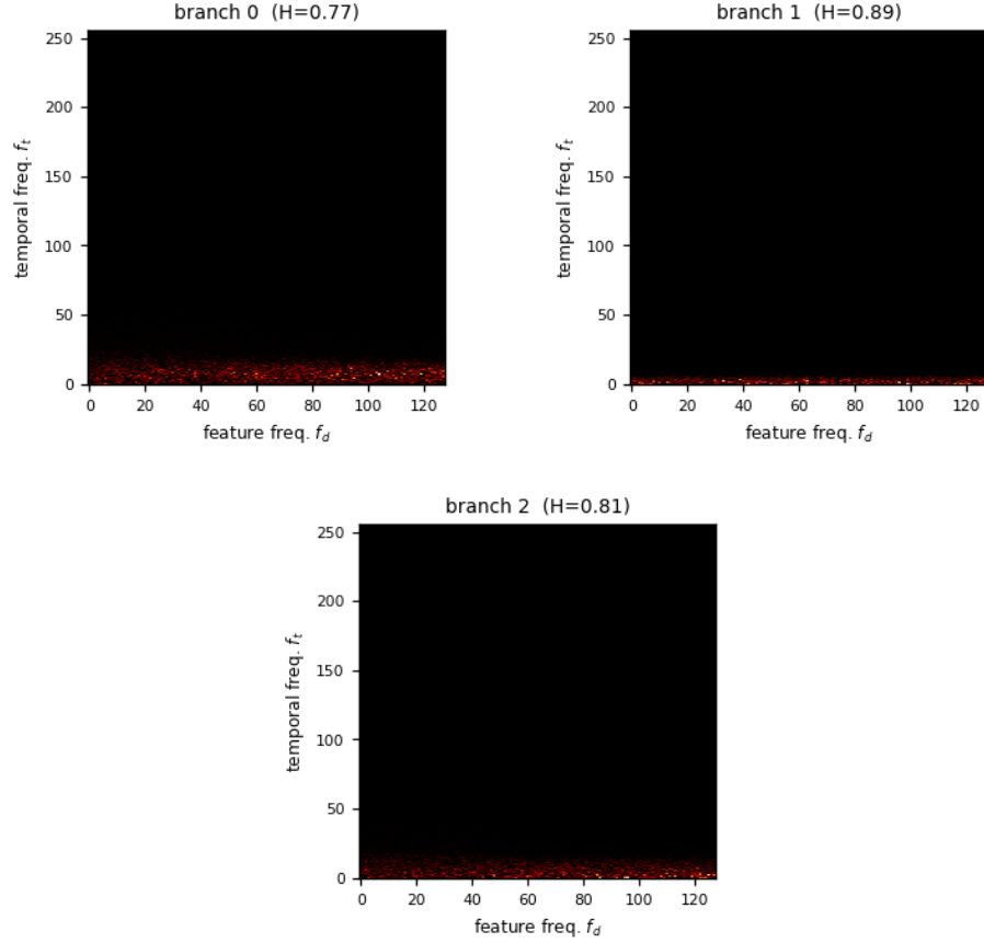
Figure 2: The static amplitude spectrum |a[f_t, f_d]| across the 3 arms of calm-d’s prismatic head - the learned grid that, inverse-transformed through the frozen Weyl phases, becomes the bias field. This is the heatmap the text describes: energy that settles into a low-frequency band (small f_t, f_d ) is the corpus rhythm crystallizing, while a grid that stays uniform is a field still indistinguishable from noise. Hoyer concentrations H = 0.77, 0.89, 0.81 (left to right) quantifies it on the same [0, 1] scale the prose names (1 = a single cell, 0 = uniform), computed from this very tensor by concentration() - the same value the dashboard logs live. The pink 1/f^\alpha prior lives in the frozen basis, not in these amplitudes, so the grid shown is exactly what the head exposes.
