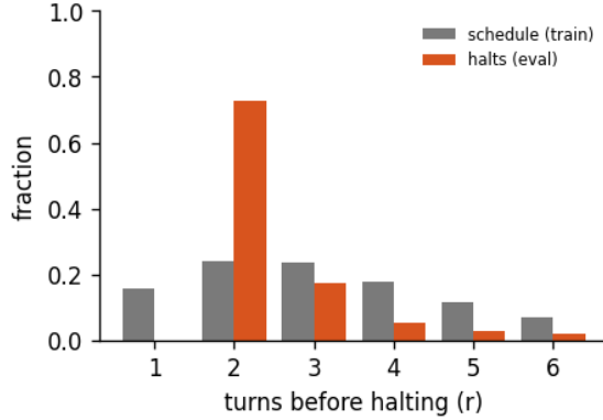
Figure 8: Halting distribution: the fraction of forward passes that stop after r turns, for the 6-turn recurrent loop of run abstractinator-j, early-halt rate 40%, mean boundary KL 0.222. schedule is the random loop-count the model trains under; halts is where the KL gate actually stops at inference. A mass pinned at the maximum (KL never collapsing) is the honest signature of a model that has not yet learned to converge early - the decision is real, not yet decisive.
