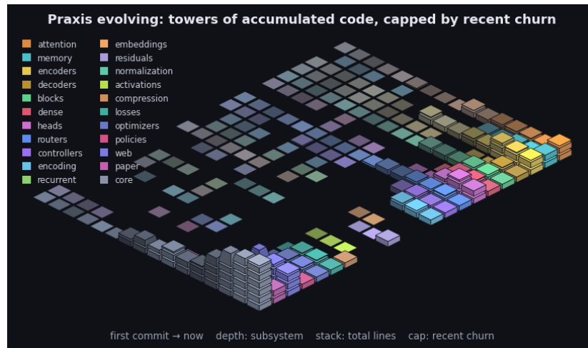
Figure 12: Praxis's git history as an isometric terrain over the last 2494 commits. Each cell is one subsystem in one time window: a stack of base blocks for its accumulated size (total lines, recency-weighted) topped by a vivid cap for that window's line churn - the standing codebase carrying the recent activity. Both are weighted by recency (the kernel the model applies to a sequence, turned on the repository): recent windows stack tall with bright caps while history thins toward the always-present prior - the low valley we roll into. Color fades from each subsystem's hue toward a neutral prior into the past, banded in phased strata over a non-linear timescale. It is the bias/variance geometry read along the frequency axis (see the project notes): loud recent corrections over the quiet, ever-present base. By recency-weighted churn the current center of gravity is core, web, paper. The framework charts the hand that builds it.
