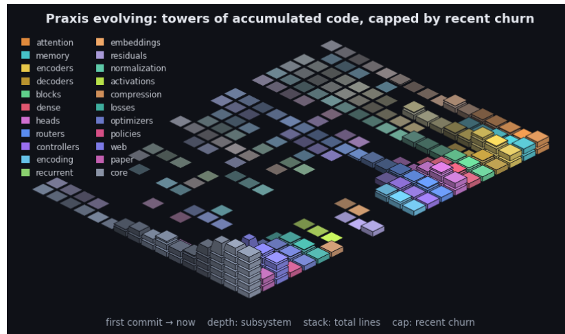
Figure 12: Praxis’s git history as an isometric terrain over the last 2487 commits. Each cell is one subsystem in one time window: a stack of base blocks for its accumulated size (total lines, recency-weighted) topped by a vivid cap for that window’s line churn - the standing codebase carrying the recent activity. Both are weighted by recency (the kernel the model applies to a sequence, turned on the repository): recent windows stack tall with bright caps while history thins toward the always-present prior - the low valley we roll into. Color fades from each subsystem’s hue toward a neutral prior into the past, banded in phased strata over a non-linear timescale. It is the bias/variance geometry read along the frequency axis (see the project notes): loud recent corrections over the quiet, ever-present base. By recency-weighted churn the current center of gravity is core, web, paper. The framework charts the hand that builds it.
