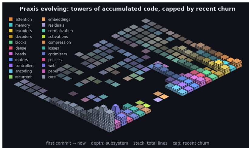
Figure 5: Praxis’s git history as an isometric terrain over the last 2348 commits. Each cell is one subsystem in one time window: a stack of base blocks for its accumulated size (total lines, recency-weighted) topped by a vivid cap for that window’s line churn - the standing codebase carrying the recent activity. Both are weighted by recency (the kernel the model applies to a sequence, turned on the repository): recent windows stack tall with bright caps while history thins toward the always-present prior - the low valley we roll into. Color fades from each subsystem’s hue toward a neutral prior into the past, banded in phased strata over a non-linear timescale. It is the bias/variance geometry read along the frequency axis (see the project notes): loud recent corrections over the quiet, ever-present base. By recency-weighted churn the current center of gravity is core, web, paper. The framework charts the hand that builds it.
