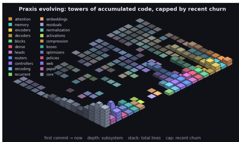
Figure 4: Praxis’s git history as an isometric terrain over the last 2316 commits. Each cell is one subsystem in one time window: a stack of base blocks for its accumulated size (total lines, recency-weighted) topped by a vivid cap for that window’s line churn - the standing codebase carrying the recent activity. Both are weighted by recency (the kernel the model applies to a sequence, turned on the repository): recent windows stack tall with bright caps while history thins toward the always-present prior - the low valley we roll into. Color fades from each subsystem’s hue toward a neutral prior into the past, banded in phased strata over a non-linear timescale. It is the bias/variance geometry read along the frequency axis (see the project notes): loud recent corrections over the quiet, ever-present base. By recency-weighted churn the current center of gravity is core, web, paper. The framework charts the hand that builds it.
