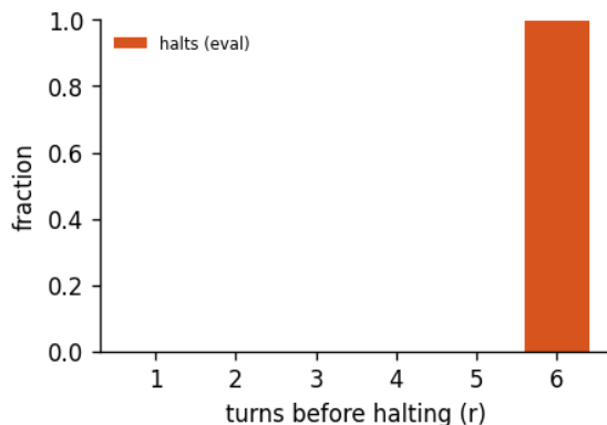
Figure 5: Halting distribution: the fraction of forward passes that stop after r turns, for the 6-turn recurrent loop of run calm-d, early-halt rate 0%, mean boundary KL 96.6. schedule is the random loop-count the model trains under; halts is where the KL gate actually stops at inference. A mass pinned at the maximum (KL never collapsing) is the honest signature of a model that has not yet learned to converge early - the decision is real, not yet decisive.
