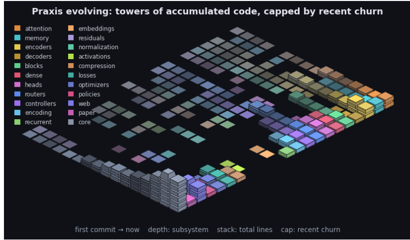
Figure 7: Praxis’s git history as an isometric terrain over the last 2223 commits. Each cell is one subsystem in one time window: a stack of base blocks for its accumulated size (total lines, recency-weighted) topped by a vivid cap for that window’s line churn - the standing codebase carrying the recent activity. Both are weighted by recency (the kernel the model applies to a sequence, turned on the repository): recent windows stack tall with bright caps while history thins toward the always-present prior - the low valley we roll into. Color fades from each subsystem’s hue toward a neutral prior into the past, banded in phased strata over a non-linear timescale. It is the bias/variance geometry read along the frequency axis (see the project notes): loud recent corrections over the quiet, ever-present base. By recency-weighted churn the current center of gravity is core, web, encoders. The framework charts the hand that builds it.
