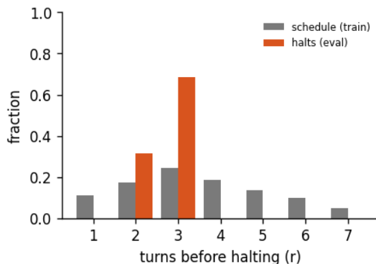
Figure 7: Halting distribution: the fraction of forward passes that stop after r turns, for the 7-turn recurrent loop of run abstractinator-b, early-halt rate 37%, mean boundary KL 0.279. schedule is the random loop-count the model trains under; halts is where the KL gate actually stops at inference. A mass pinned at the maximum (KL never collapsing) is the honest signature of a model that has not yet learned to converge early - the decision is real, not yet decisive.
