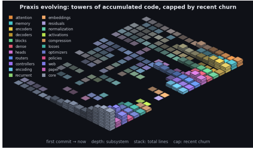
Figure 11: Praxis’s git history as an isometric terrain over the last 2414 commits. Each cell is one subsystem in one time window: a stack of base blocks for its accumulated size (total lines, recency-weighted) topped by a vivid cap for that window’s line churn - the standing codebase carrying the recent activity. Both are weighted by recency (the kernel the model applies to a sequence, turned on the repository): recent windows stack tall with bright caps while history thins toward the always-present prior - the low valley we roll into. Color fades from each subsystem’s hue toward a neutral prior into the past, banded in phased strata over a non-linear timescale. It is the bias/variance geometry read along the frequency axis (see the project notes): loud recent corrections over the quiet, ever-present base. By recency-weighted churn the current center of gravity is core, web, paper. The framework charts the hand that builds it.
