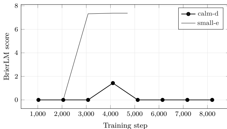
Figure 5: BrierLM across the 2 most recent experiments with comparable validation curves; the leading run (calm-d) is drawn in bold. Generated from run logs - metrics that are not comparable across families (token loss vs. byte bits-per-byte vs. codec/CALM BrierLM) are excluded by construction, so the curves on this axis mean the same thing.
