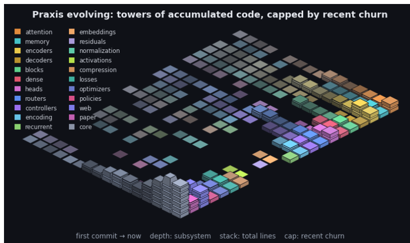
Figure 4: Praxis’s git history as an isometric terrain over the last 2290 commits. Each cell is one subsystem in one time window: a stack of base blocks for its accumulated size (total lines, recency-weighted) topped by a vivid cap for that window’s line churn - the standing codebase carrying the recent activity. Both are weighted by recency (the kernel the model applies to a sequence, turned on the repository): recent windows stack tall with bright caps while history thins toward the always-present prior - the low valley we roll into. Color fades from each subsystem’s hue toward a neutral prior into the past, banded in phased strata over a non-linear timescale. It is the bias/variance geometry read along the frequency axis (see the project notes): loud recent corrections over the quiet, ever-present base. By recency-weighted churn the current center of gravity is core, web, paper. The framework charts the hand that builds it.
