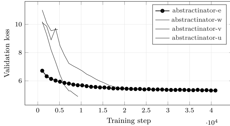
Figure 10: Validation Loss across the 4 most recent experiments with comparable validation curves; the current experiment (abstractinator-e) is drawn in bold. Bold marks which run this build is reporting on , not which run scores best. The curves end wherever each run stopped, so they are at different points along their own training, and their endpoints are not a ranking. Generated from run logs - metrics that are not comparable across families (token loss vs. byte bits-per-byte vs. codec/CALM BrierLM) are excluded by construction, so the curves on this axis mean the same thing.
