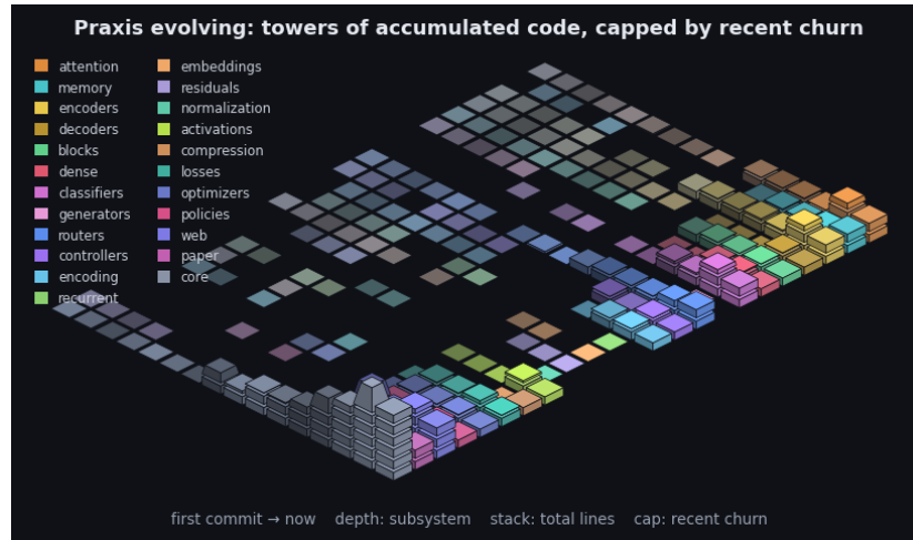
Figure 9: Praxis’s git history as an isometric terrain over the last 2637 commits. Each cell is one subsystem in one time window: a stack of base blocks for its accumulated size (total lines, recency-weighted) topped by a vivid cap for that window’s line churn - the standing codebase carrying the recent activity. Both are weighted by recency (the kernel the model applies to a sequence, turned on the repository): recent windows stack tall with bright caps while history thins toward the always-present prior - the low valley we roll into. Color fades from each subsystem’s hue toward a neutral prior into the past, banded in phased strata over a non-linear timescale. It is the bias/variance geometry read along the frequency axis (see the project notes): loud recent corrections over the quiet, ever-present base. By recency-weighted churn the current center of gravity is core, web, encoders. The framework charts the hand that builds it.
