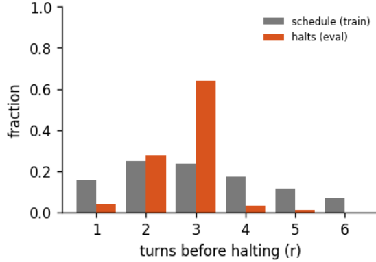
Figure 9: Halting distribution: the fraction of forward passes that stop after r turns, for the 6-turn recurrent loop of run byte-latent-a, early-halt rate 37%, mean boundary KL 0.0158. schedule is the random loop-count the model trains under; halts is where the KL gate actually stops at inference. A mass pinned at the maximum (KL never collapsing) is the honest signature of a model that has not yet learned to converge early - the decision is real, not yet decisive.
