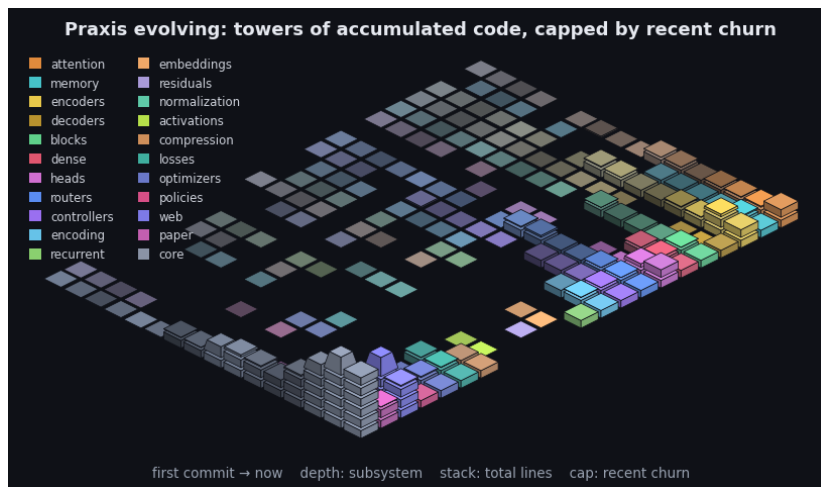
Figure 4: Praxis’s git history as an isometric terrain over the last 2294 commits. Each cell is one subsystem in one time window: a stack of base blocks for its accumulated size (total lines, recency-weighted) topped by a vivid cap for that window’s line churn - the standing codebase carrying the recent activity. Both are weighted by recency (the kernel the model applies to a sequence, turned on the repository): recent windows stack tall with bright caps while history thins toward the always-present prior - the low valley we roll into. Color fades from each subsystem’s hue toward a neutral prior into the past, banded in phased strata over a non-linear timescale. It is the bias/variance geometry read along the frequency axis (see the project notes): loud recent corrections over the quiet, ever-present base. By recency-weighted churn the current center of gravity is core, web, paper. The framework charts the hand that builds it.
