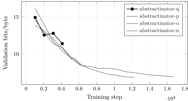
Figure 13: Bits per Byte across the 4 most recent experiments with comparable validation curves; the current experiment (abstractinator-q) is drawn in bold. Bold marks which run this build is reporting on , not which run scores best. The curves end wherever each run stopped, so they are at different points along their own training, and their endpoints are not a ranking. Generated from run logs - metrics that are not comparable across families (token loss vs. byte bits-per-byte vs. codec/CALM BrierLM) are excluded by construction, so the curves on this axis mean the same thing.
