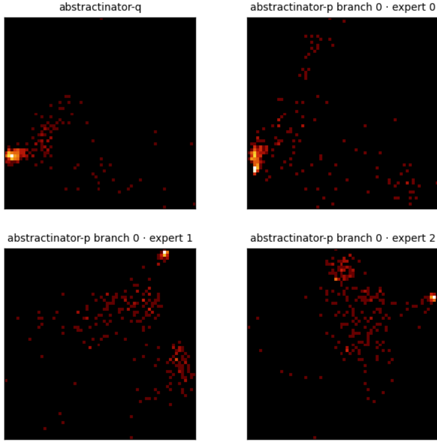
Figure 11: Center PCA density for the 4 most recent crystal-head runs (abstractinator-q, abstractinator-p (branch 0 · expert 0), abstractinator-p (branch 0 · expert 1), abstractinator-p (branch 0 · expert 2)). Each panel is the top-2 PCA projection of a head’s vocabulary centers, binned to a 64 \times 64 density grid (log color) - the same snapshot the dashboard renders live. Different runs settle into structurally different geometries, not noise.
