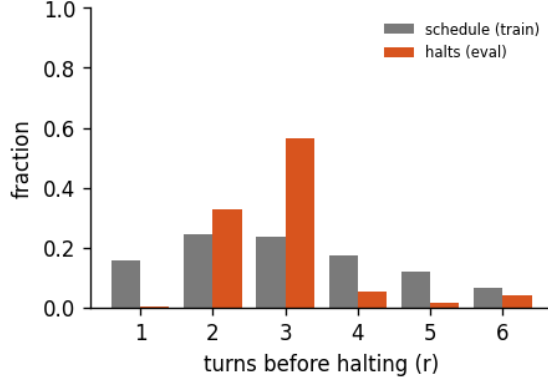
Figure 8: Halting distribution: the fraction of forward passes that stop after r turns, for the 6-turn recurrent loop of run abstractinator-q, early-halt rate 34%, mean boundary KL 0.212. schedule is the random loop-count the model trains under; halts is where the KL gate actually stops at inference. A mass pinned at the maximum (KL never collapsing) is the honest signature of a model that has not yet learned to converge early - the decision is real, not yet decisive.
