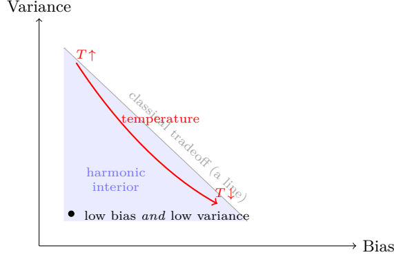
Figure 1: Bias and variance as orthogonal coordinates. Classically a model must sit somewhere on the gray line: less of one means more of the other. When a static spectrum supplies bias and an input-conditional modulation supplies variance, the two decouple, and the interior (shaded) becomes reachable - lower bias and lower variance than any point on the line. Temperature is a path through this space, not noise added at a fixed point.
