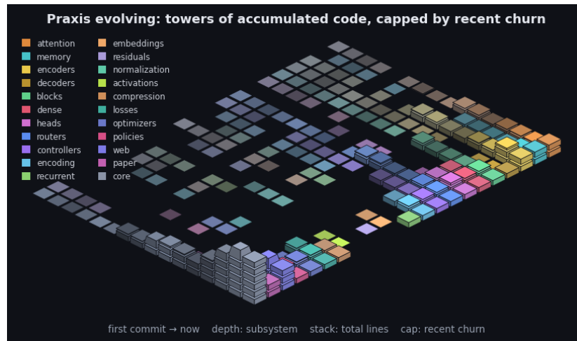
Figure 4: Praxis’s git history as an isometric terrain over the last 2263 commits. Each cell is one subsystem in one time window: a stack of base blocks for its accumulated size (total lines, recency-weighted) topped by a vivid cap for that window’s line churn - the standing codebase carrying the recent activity. Both are weighted by recency (the kernel the model applies to a sequence, turned on the repository): recent windows stack tall with bright caps while history thins toward the always-present prior - the low valley we roll into. Color fades from each subsystem’s hue toward a neutral prior into the past, banded in phased strata over a non-linear timescale. It is the bias/variance geometry read along the frequency axis (see the project notes): loud recent corrections over the quiet, ever-present base. By recency-weighted churn the current center of gravity is core, web, encoders. The framework charts the hand that builds it.
