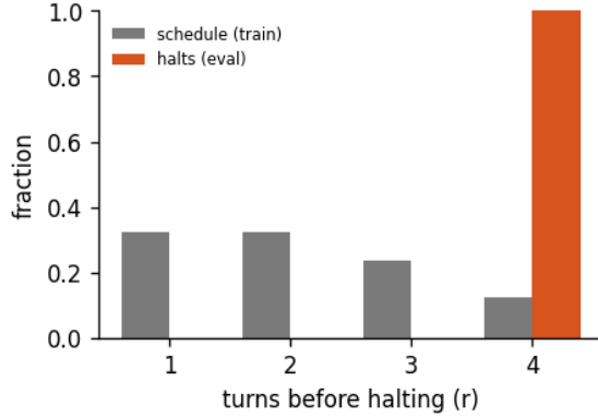
Figure 3: Halting distribution: the fraction of forward passes that stop after r turns, for the 4-turn recurrent loop of run calm-f, early-halt rate 0%, mean boundary KL 2.34. schedule is the random loop-count the model trains under; halts is where the KL gate actually stops at inference. A mass pinned at the maximum (KL never collapsing) is the honest signature of a model that has not yet learned to converge early - the decision is real, not yet decisive.
