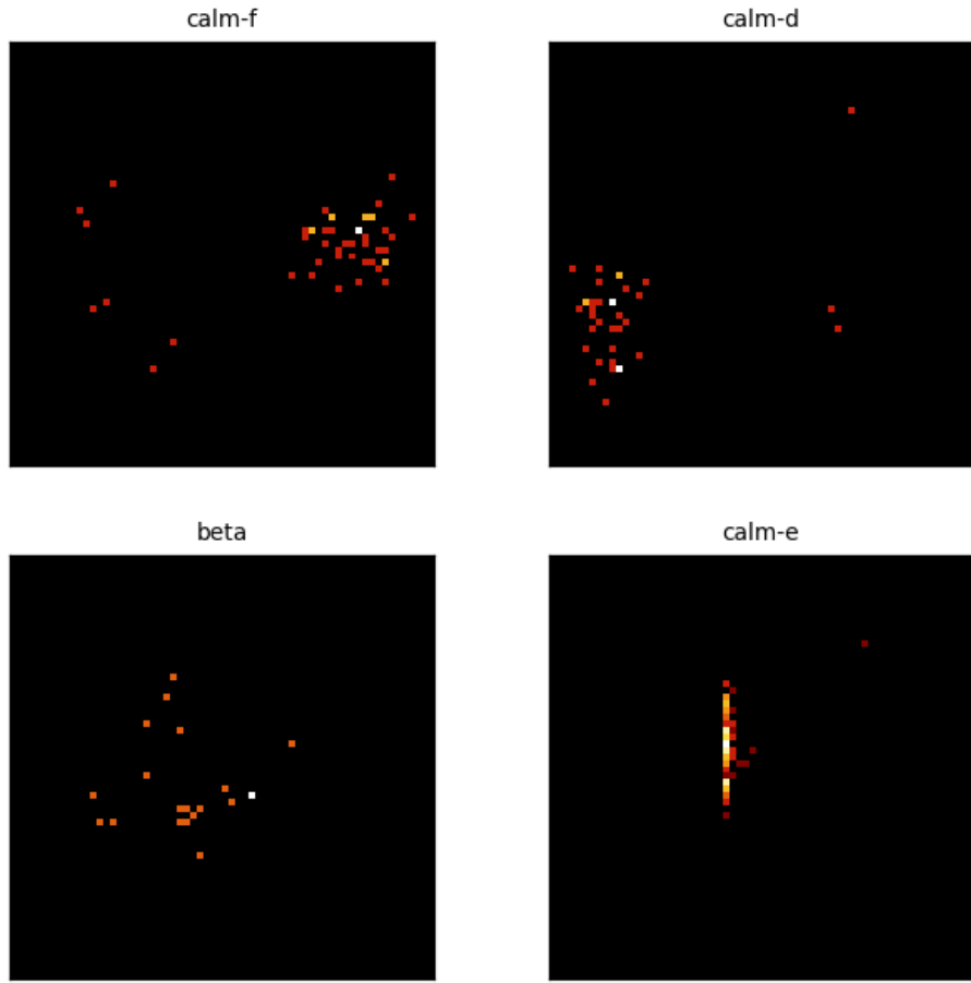
Figure 2: Center PCA density for the 4 most recent crystal-head runs (calm-f, calm-d, beta, calm-e). Each panel is the top-2 PCA projection of a head's vocabulary centers, binned to a 64 \times 64 density grid (log color) - the same snapshot the dashboard renders live. Different runs settle into structurally different geometries, not noise.
