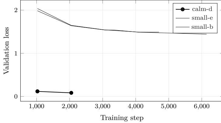
Figure 7: Validation Loss across the 3 most recent experiments with comparable validation curves; the leading run (calm-d) is drawn in bold. Generated from run logs - metrics that are not comparable across families (token loss vs. byte bits-per-byte vs. codec/CALM BrierLM) are excluded by construction, so the curves on this axis mean the same thing.
