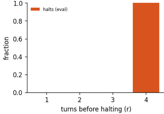
Figure 4: Halting distribution: the fraction of forward passes that stop after r turns, for the 4-turn recurrent loop of run calm-f, early-halt rate 0%, mean boundary KL 3.02. schedule is the random loop-count the model trains under; halts is where the KL gate actually stops at inference. A mass pinned at the maximum (KL never collapsing) is the honest signature of a model that has not yet learned to converge early - the decision is real, not yet decisive.
