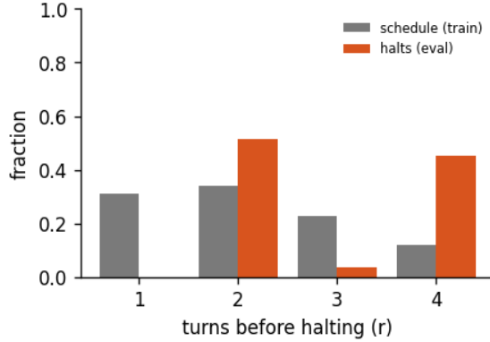
Figure 2: Halting distribution: the fraction of forward passes that stop after r turns, for the 4-turn recurrent loop of run calm-d-1, early-halt rate 22%, mean boundary KL 0.0813. schedule is the random loop-count the model trains under; halts is where the KL gate actually stops at inference. A mass pinned at the maximum (KL never collapsing) is the honest signature of a model that has not yet learned to converge early - the decision is real, not yet decisive.
