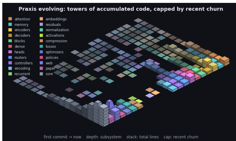
Figure 4: Praxis’s git history as an isometric terrain over the last 2344 commits. Each cell is one subsystem in one time window: a stack of base blocks for its accumulated size (total lines, recency-weighted) topped by a vivid cap for that window’s line churn - the standing codebase carrying the recent activity. Both are weighted by recency (the kernel the model applies to a sequence, turned on the repository): recent windows stack tall with bright caps while history thins toward the always-present prior - the low valley we roll into. Color fades from each subsystem’s hue toward a neutral prior into the past, banded in phased strata over a non-linear timescale. It is the bias/variance geometry read along the frequency axis (see the project notes): loud recent corrections over the quiet, ever-present base. By recency-weighted churn the current center of gravity is core, web, paper. The framework charts the hand that builds it.
