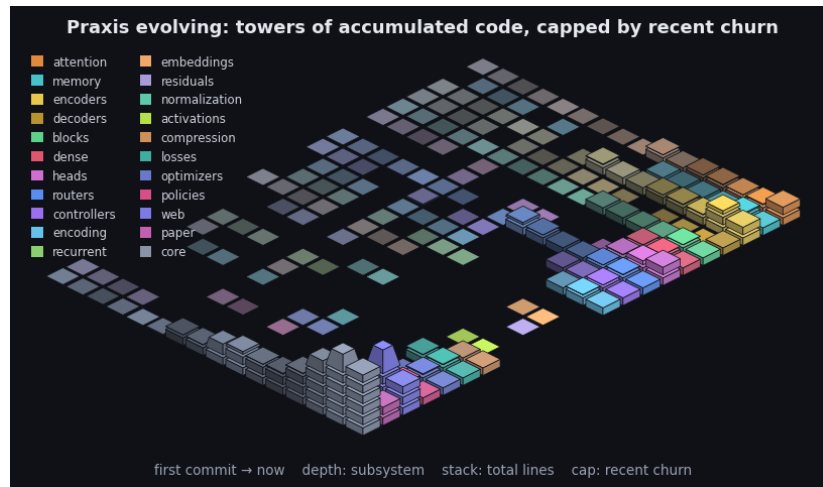
Figure 10: Praxis's git history as an isometric terrain over the last 2385 commits. Each cell is one subsystem in one time window: a stack of base blocks for its accumulated size (total lines, recency-weighted) topped by a vivid cap for that window's line churn - the standing codebase carrying the recent activity. Both are weighted by recency (the kernel the model applies to a sequence, turned on the repository): recent windows stack tall with bright caps while history thins toward the always-present prior - the low valley we roll into. Color fades from each subsystem's hue toward a neutral prior into the past, banded in phased strata over a non-linear timescale. It is the bias/variance geometry read along the frequency axis (see the project notes): loud recent corrections over the quiet, ever-present base. By recency-weighted churn the current center of gravity is core, web, paper. The framework charts the hand that builds it.
