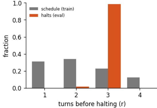
Figure 6: Halting distribution: the fraction of forward passes that stop after r turns, for the 4-turn recurrent loop of run calm-d-1, early-halt rate 34%, mean boundary KL 0.294. schedule is the random loop-count the model trains under; halts is where the KL gate actually stops at inference. A mass pinned at the maximum (KL never collapsing) is the honest signature of a model that has not yet learned to converge early - the decision is real, not yet decisive.
