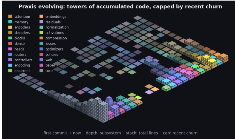
Figure 4: Praxis’s git history as an isometric terrain over the last 2335 commits. Each cell is one subsystem in one time window: a stack of base blocks for its accumulated size (total lines, recency-weighted) topped by a vivid cap for that window’s line churn - the standing codebase carrying the recent activity. Both are weighted by recency (the kernel the model applies to a sequence, turned on the repository): recent windows stack tall with bright caps while history thins toward the always-present prior - the low valley we roll into. Color fades from each subsystem’s hue toward a neutral prior into the past, banded in phased strata over a non-linear timescale. It is the bias/variance geometry read along the frequency axis (see the project notes): loud recent corrections over the quiet, ever-present base. By recency-weighted churn the current center of gravity is core, web, paper. The framework charts the hand that builds it.
