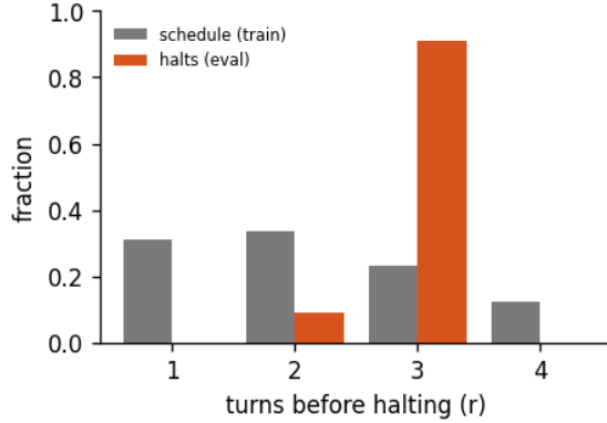
Figure 2: Halting distribution: the fraction of forward passes that stop after r turns, for the 4-turn recurrent loop of run calm-d, early-halt rate 34%, mean boundary KL 0.123. schedule is the random loop-count the model trains under; halts is where the KL gate actually stops at inference. A mass pinned at the maximum (KL never collapsing) is the honest signature of a model that has not yet learned to converge early - the decision is real, not yet decisive.
