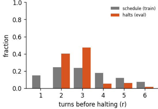
Figure 8: Halting distribution: the fraction of forward passes that stop after r turns, for the 6-turn recurrent loop of run abstractinator-1, early-halt rate 35%, mean boundary KL 0.171. schedule is the random loop-count the model trains under; halts is where the KL gate actually stops at inference. A mass pinned at the maximum (KL never collapsing) is the honest signature of a model that has not yet learned to converge early - the decision is real, not yet decisive.
