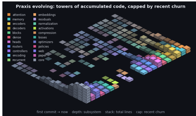
Figure 12: Praxis's git history as an isometric terrain over the last 2503 commits. Each cell is one subsystem in one time window: a stack of base blocks for its accumulated size (total lines, recency-weighted) topped by a vivid cap for that window's line churn - the standing codebase carrying the recent activity. Both are weighted by recency (the kernel the model applies to a sequence, turned on the repository): recent windows stack tall with bright caps while history thins toward the always-present prior - the low valley we roll into. Color fades from each subsystem's hue toward a neutral prior into the past, banded in phased strata over a non-linear timescale. It is the bias/variance geometry read along the frequency axis (see the project notes): loud recent corrections over the quiet, ever-present base. By recency-weighted churn the current center of gravity is core, web, paper. The framework charts the hand that builds it.
